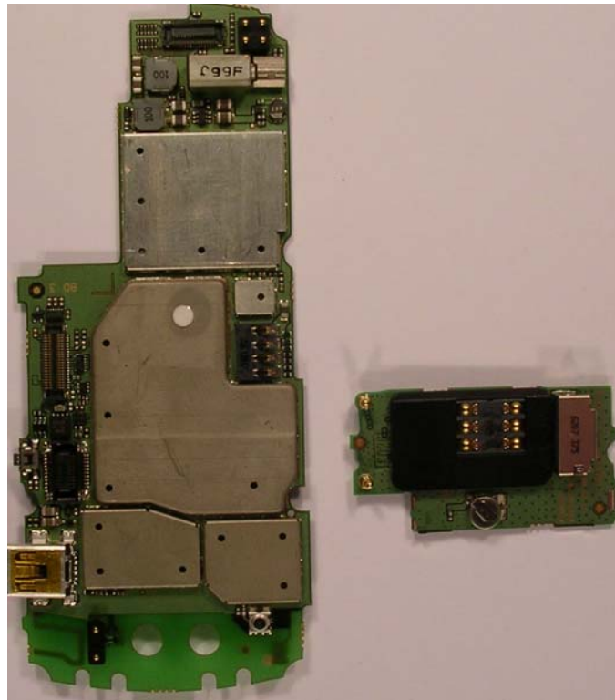
Main Board (Side A) With Shields and daughter board on the side
