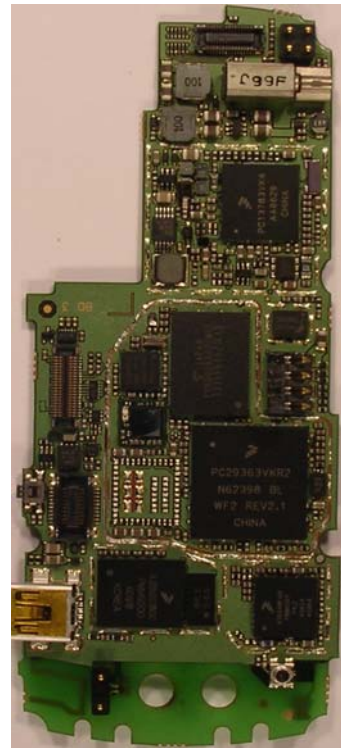
PCB (side A) With no Shields
