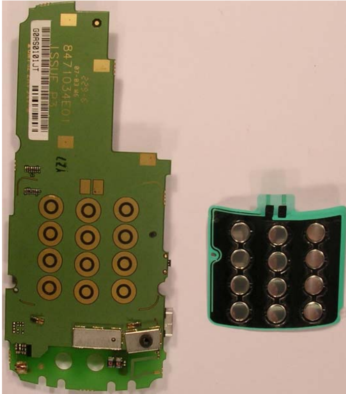
PCB (side B) and popples (flipped) on the side
