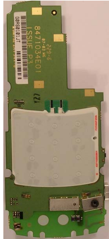
PCB (side B) and popples on PCB
