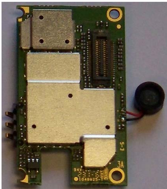
Main Board Bottom With Shields
