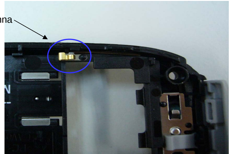
Bottom view of Bluetooth antenna
