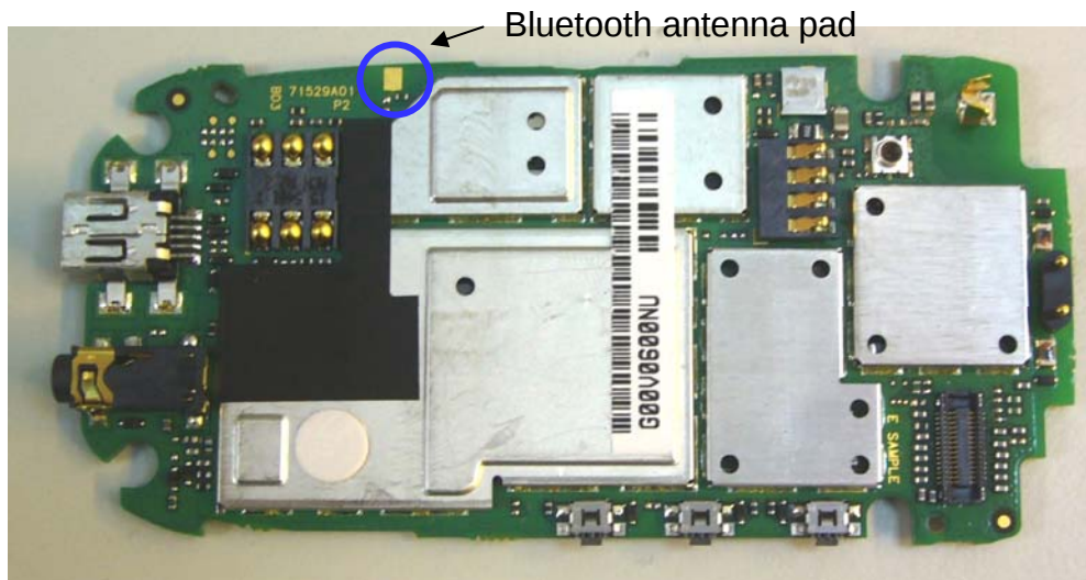
PCB board
