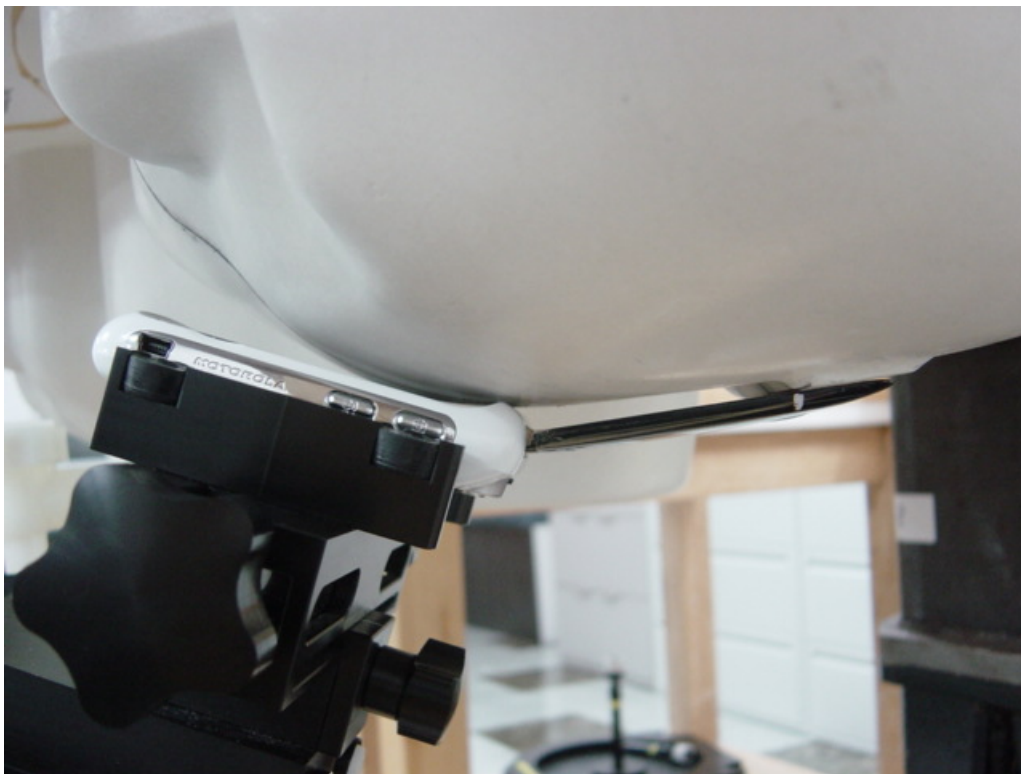
Figure 5. Phone Against the Head Phantom (Cheek Touch)
