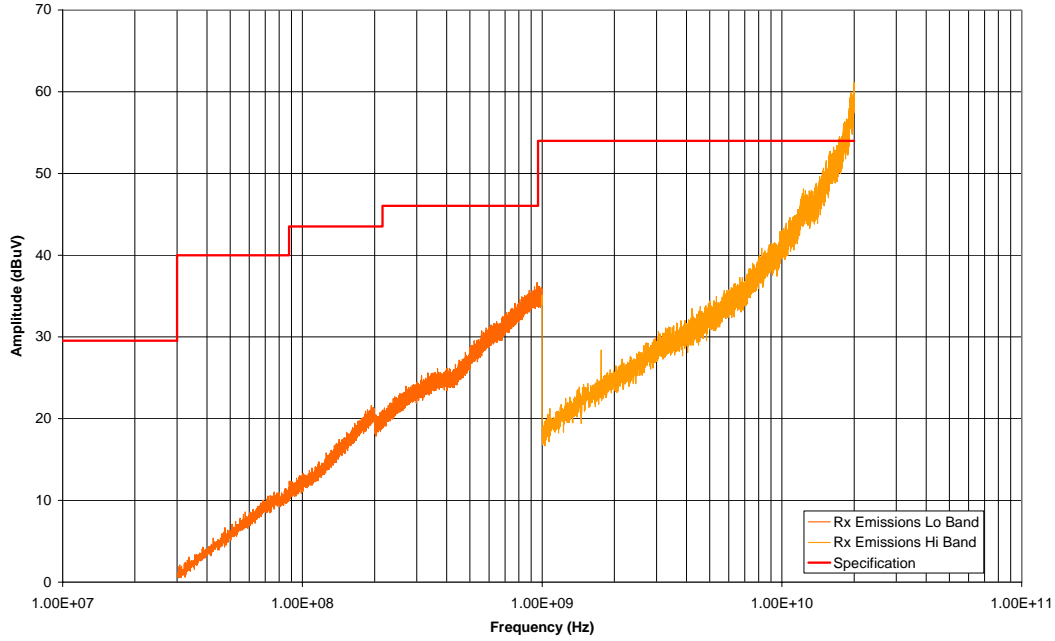
Radiated Emissions Per FCC CFR 47 Part 15.209 CDMA 800
