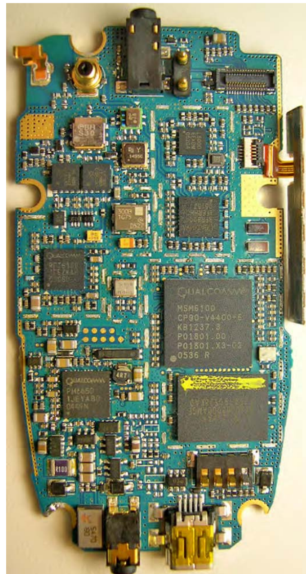
Main Board Bottom without Shields
