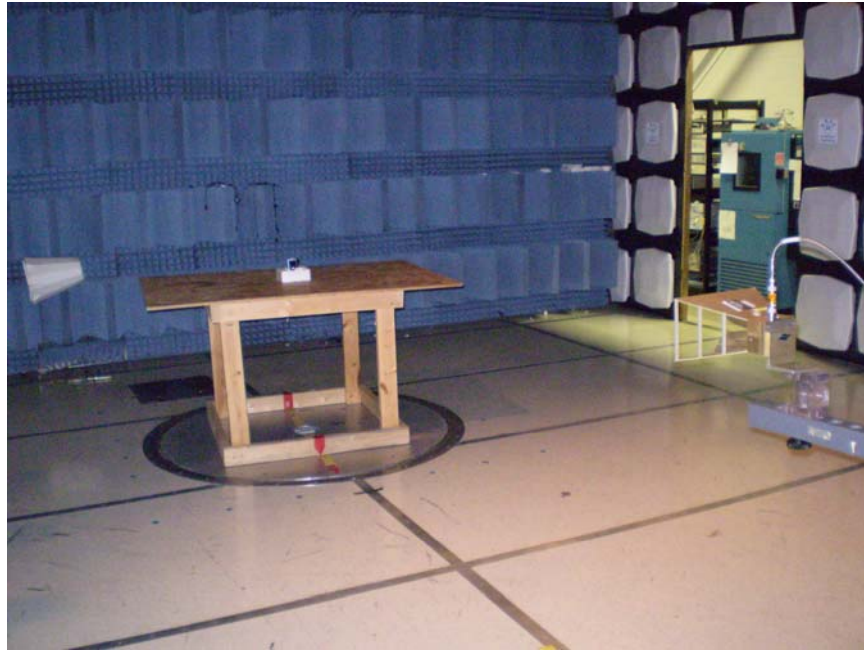
A.1 Radiated Emissions Measurement
