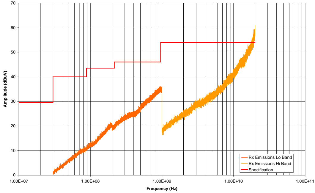
Radiated Emissions Per FCC CFR 47 Part 15.209 PCS Channel 661 - Rx Mode
