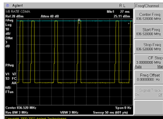
Figure 26 Zero-Span Plots
