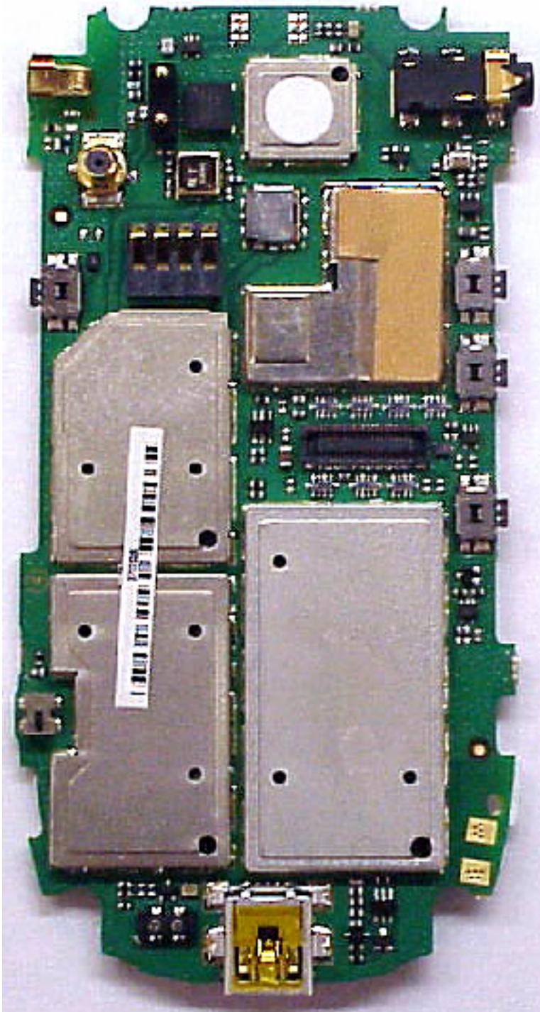
Main Board (shields on)
