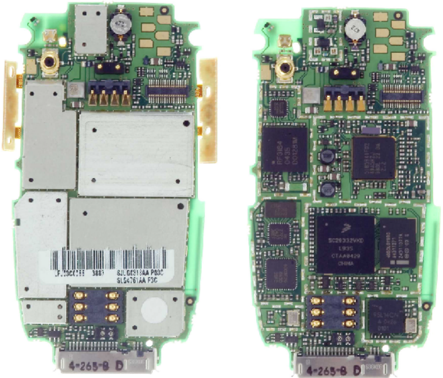
Rear Views
