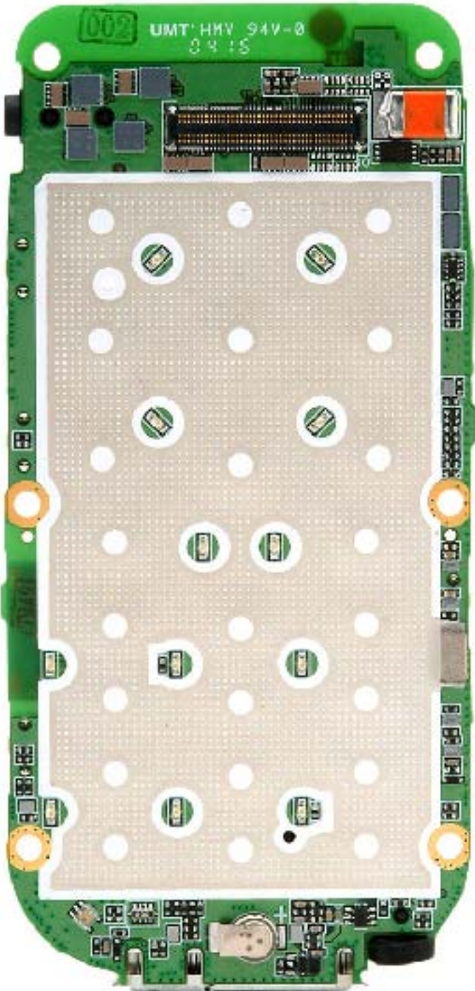
Main Board Front View with Keypad
