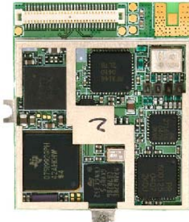
RF Module Rear View Without Shield
