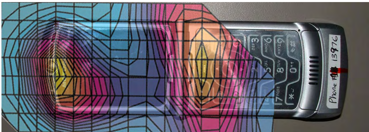
Figure 4. Typical 1900MHz GSM Head Adjacent Contour Overlaid on Phone (15 ° Tilt)
