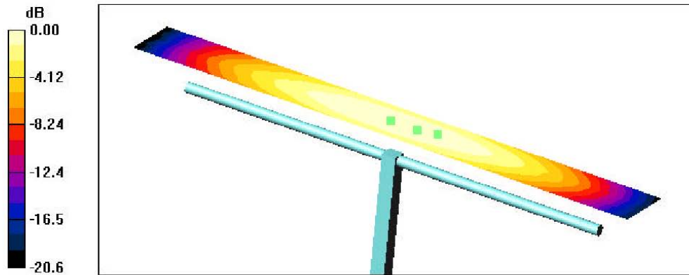
0 dB = 0.503A/m
