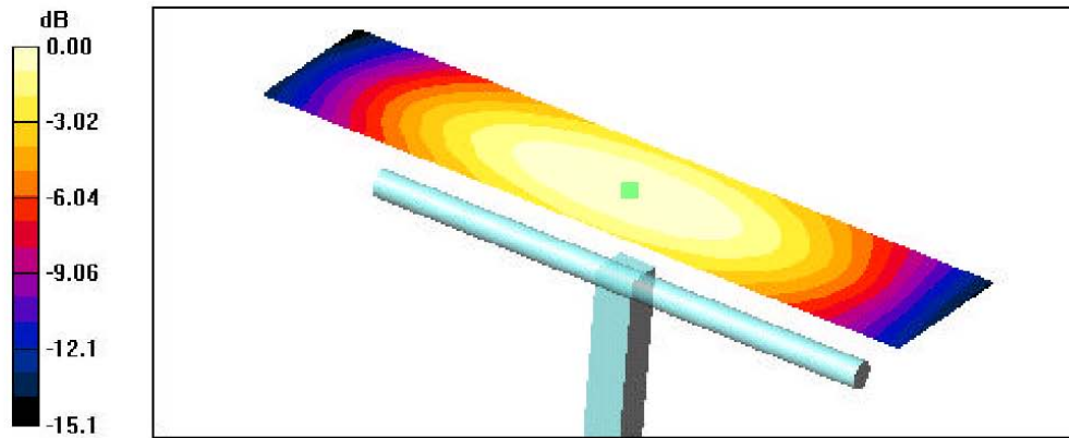
0 dB = 0.448A/m
