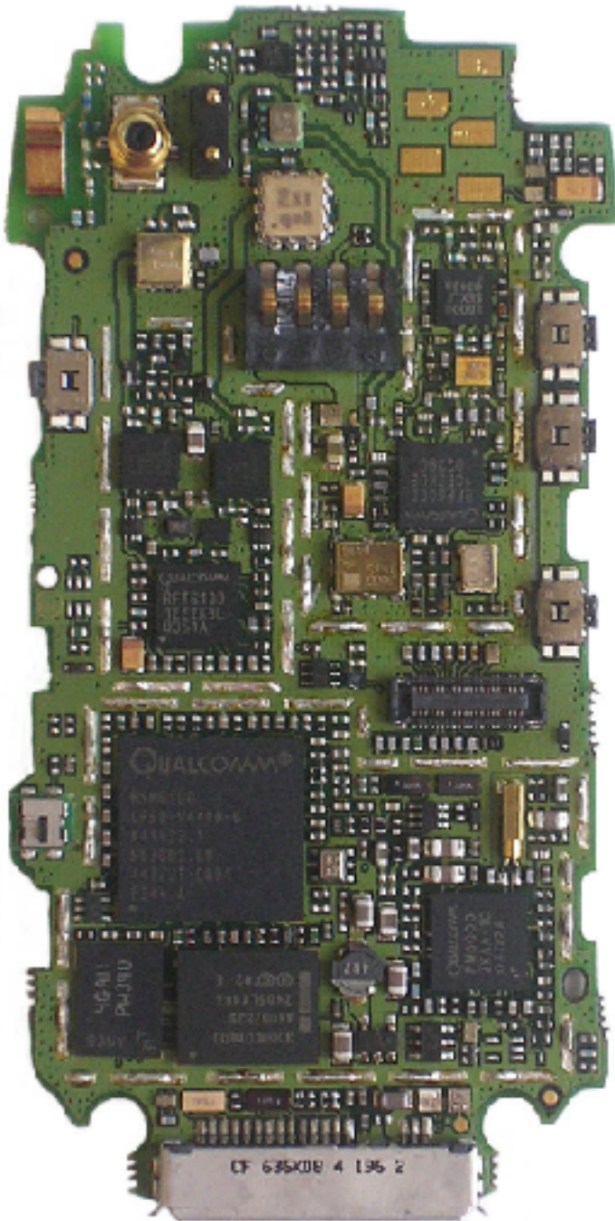
Rear View
