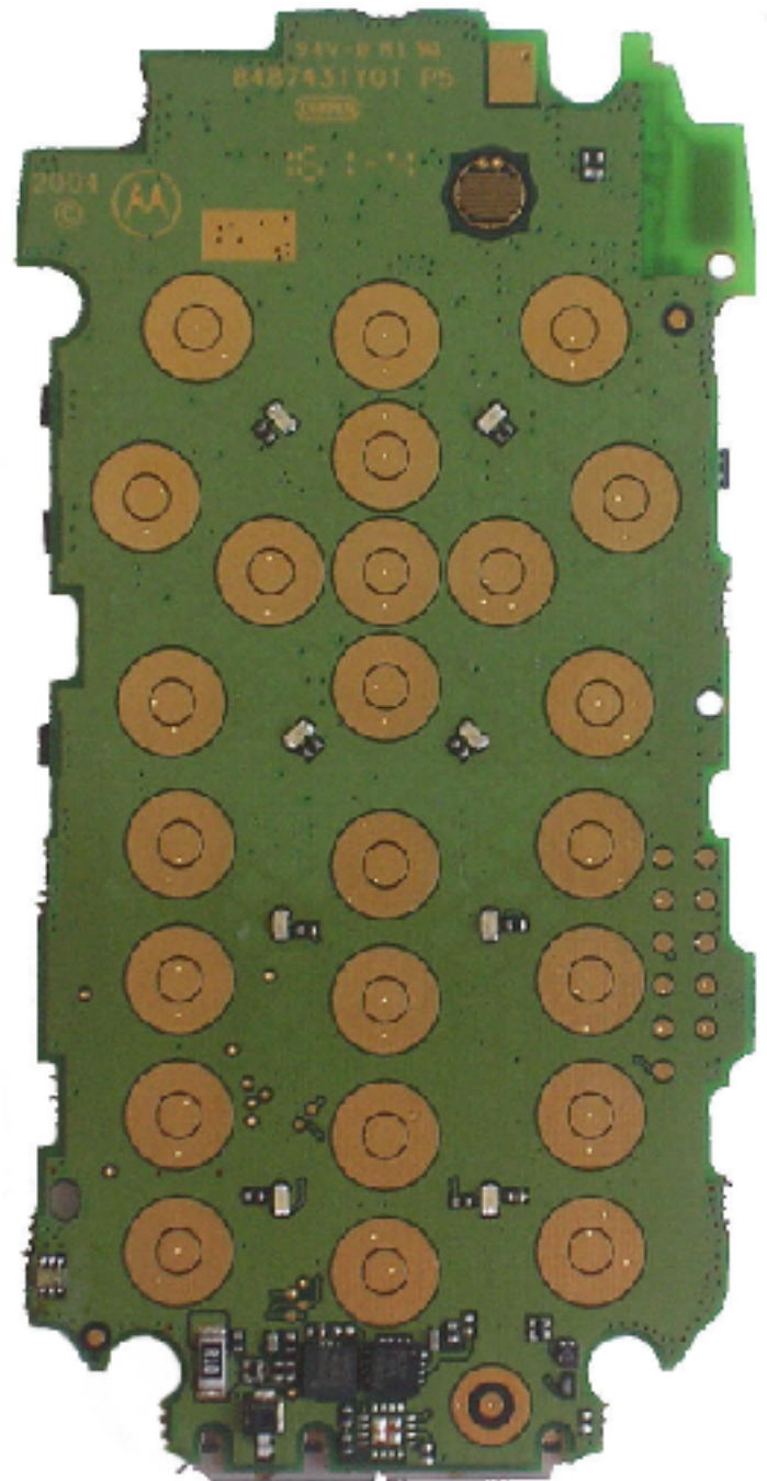
Front View
