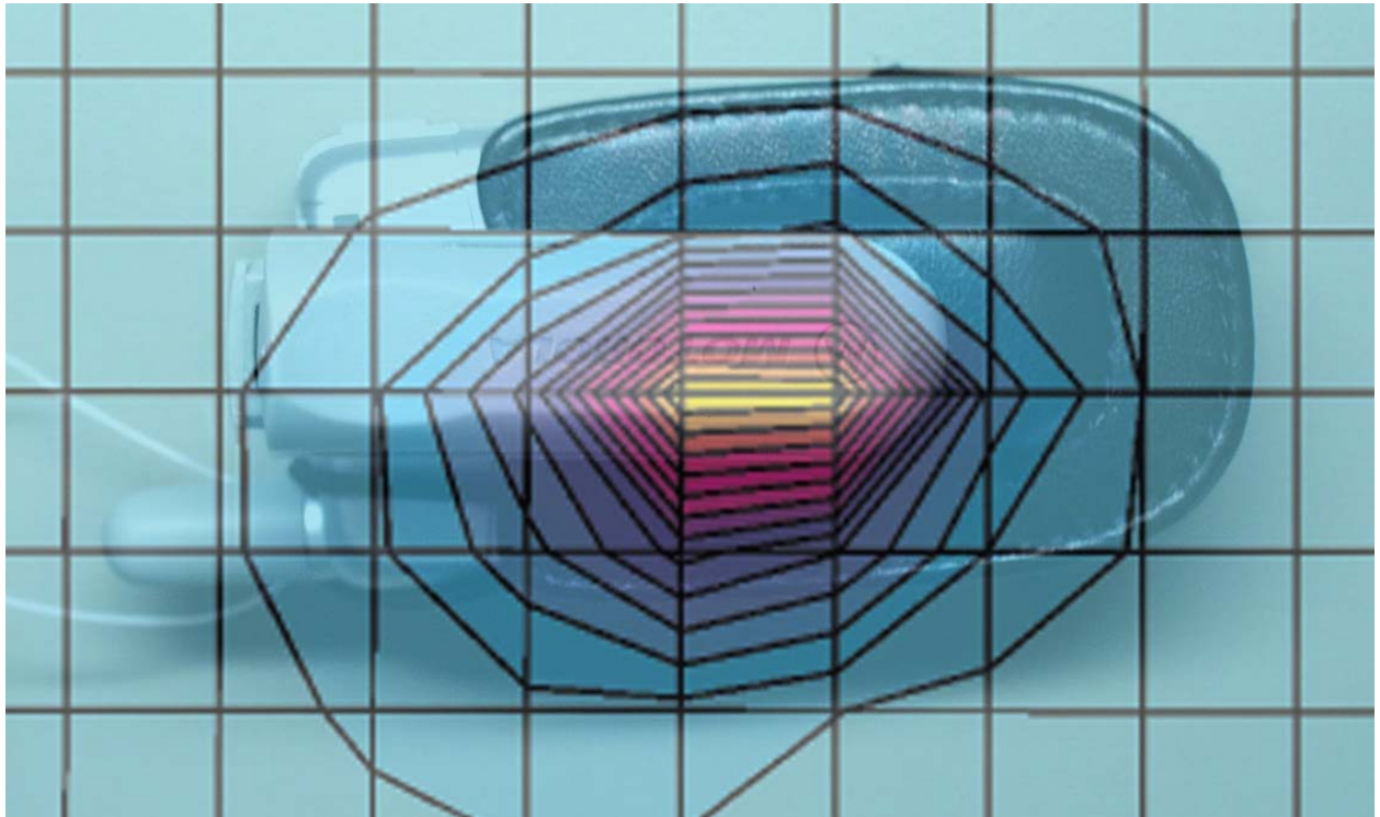
Figure 3. Typical 1900MHz Body-Worn Contour Overlaid on Phone with Antenna Fixed
