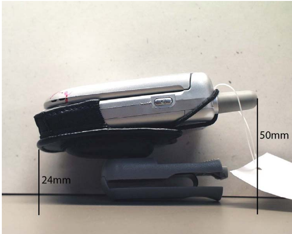
Figure 8. Side view, VLV2203 case with SYN8763A clip
