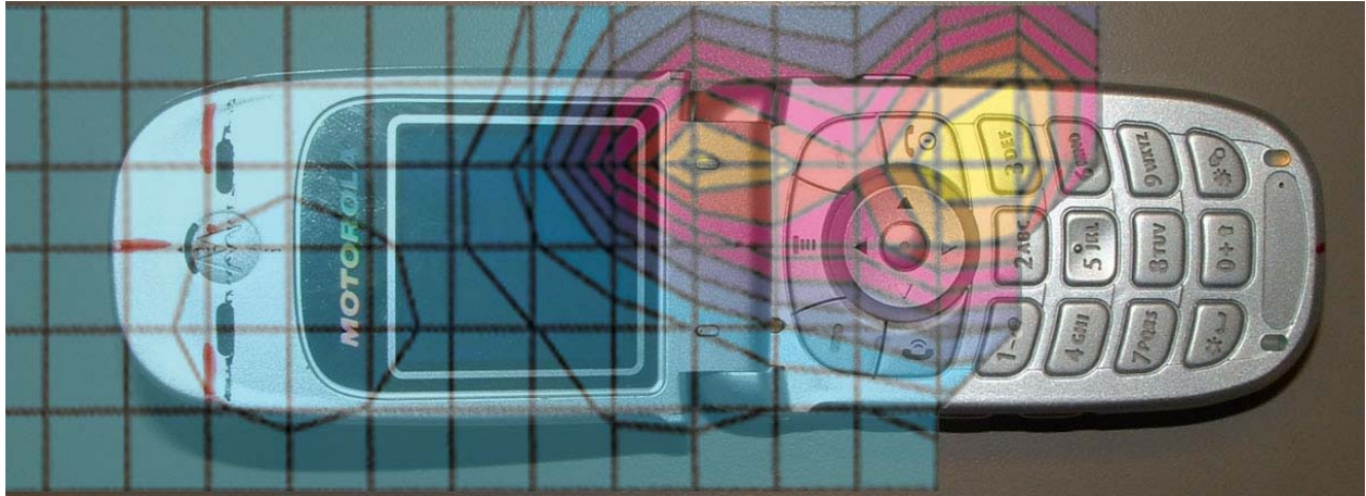
Figure 1. Typical 1900MHz Head Adjacent Contour Overlaid on Phone (Cheek Touch)
