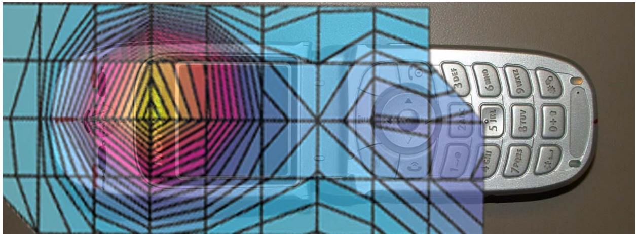
Figure 2. Typical 1900MHz Head Adjacent Contour Overlaid on Phone (15° Tilt)
