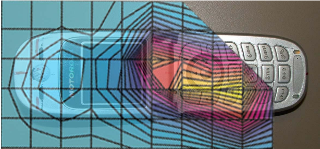
Figure 3. Typical 1900MHz Head Adjacent Contour Overlaid on Phone (Cheek Touch)
