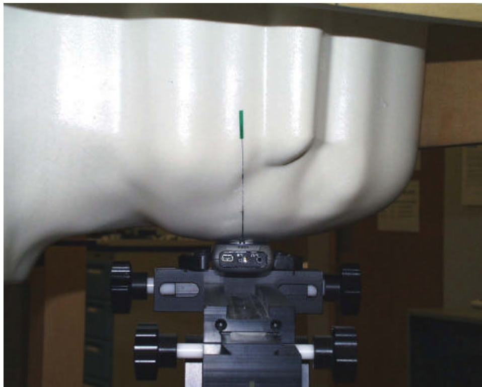
Figure 7. Phone Against the Head Phantom (Front View - Cheek Touch)
