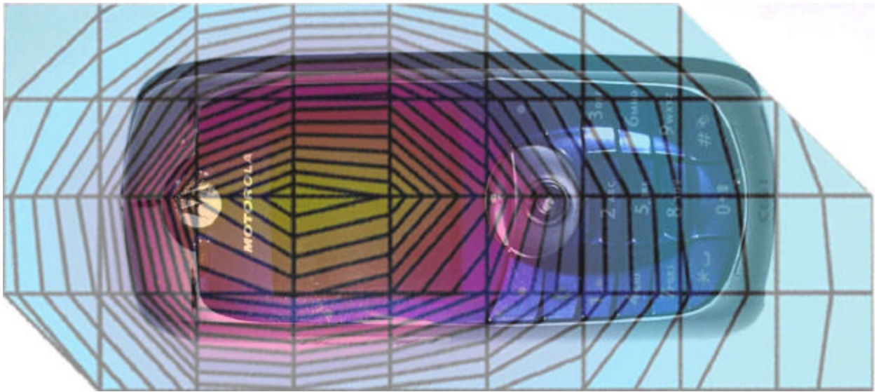
Figure 2. 850MHz Left Head Adjacent Contour Overlaid on Phone with Antenna Fixed (15 ° Tilt)
