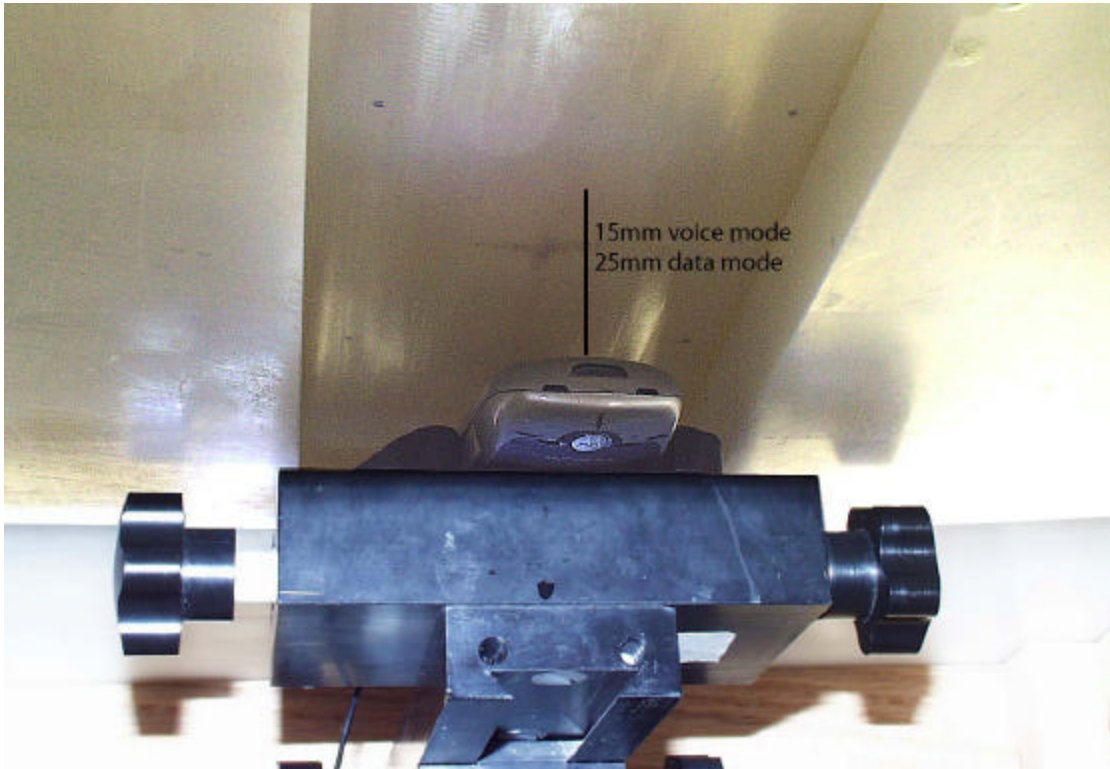
Figure 11. Body Worn Testing
