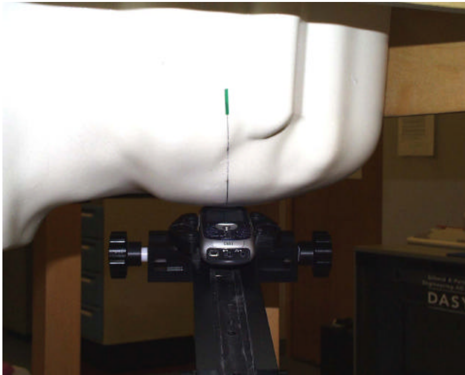
Figure 9. Phone Against the Head Phantom (Front View – 15°Tilt)
