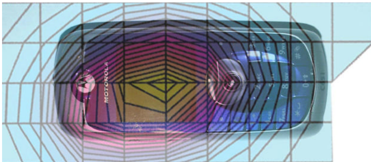
Figure 3. Typical 850MHz Right Head Adjacent Contour Overlaid on Phone with Antenna Fixed (Cheek Touch)
