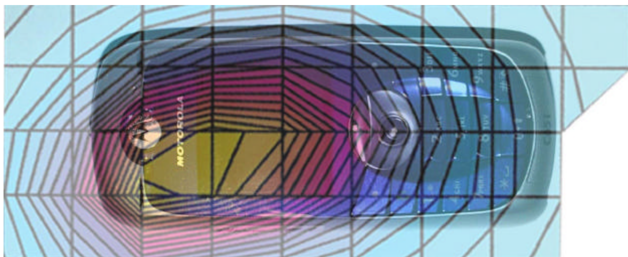
Figure 4. Typical 850MHz Left Head Adjacent Contour Overlaid on Phone with Antenna Fixed (15 ° Tilt)
