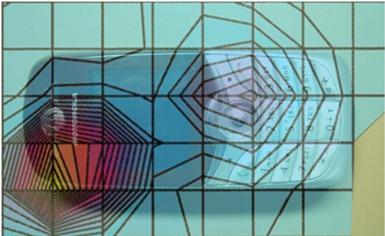
Figure 4. Typical 1900MHz Right Head Adjacent Contour Overlaid on Phone with Antenna Fixed (Cheek Touch)
