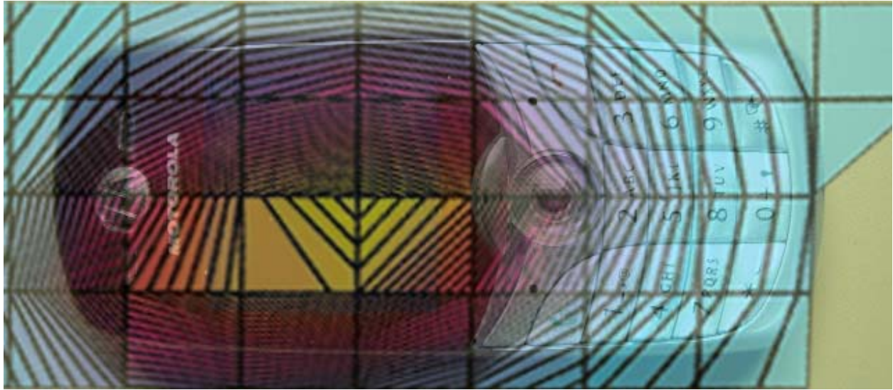
Figure 3. Typical 850MHz Right Head Adjacent Contour Overlaid on Phone with Antenna Fixed (Cheek Touch)
