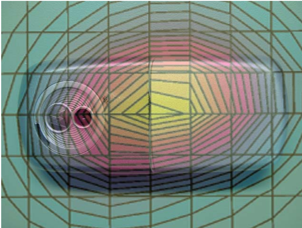
Figure 9. Typical 850 MHz Body-Worn Contour Overlaid on Phone in Voice Mode
