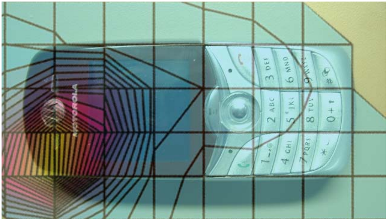
Figure 6. Typical 1900MHz Left Head Adjacent Contour Overlaid on Phone with Antenna Fixed (15 ° Tilt)
