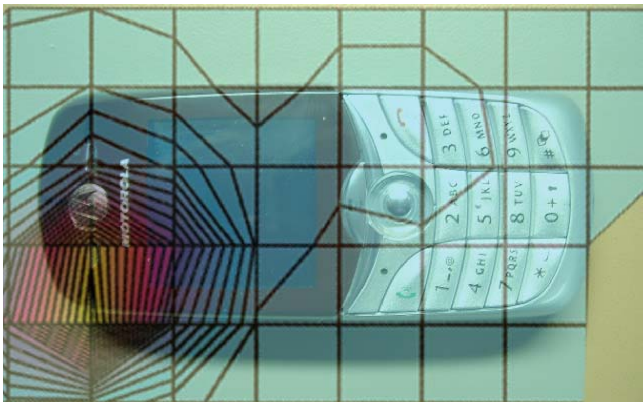
Figure 8. Typical 1900MHz Right Head Adjacent Contour Overlaid on Phone with Antenna Fixed (15 ° Tilt)
