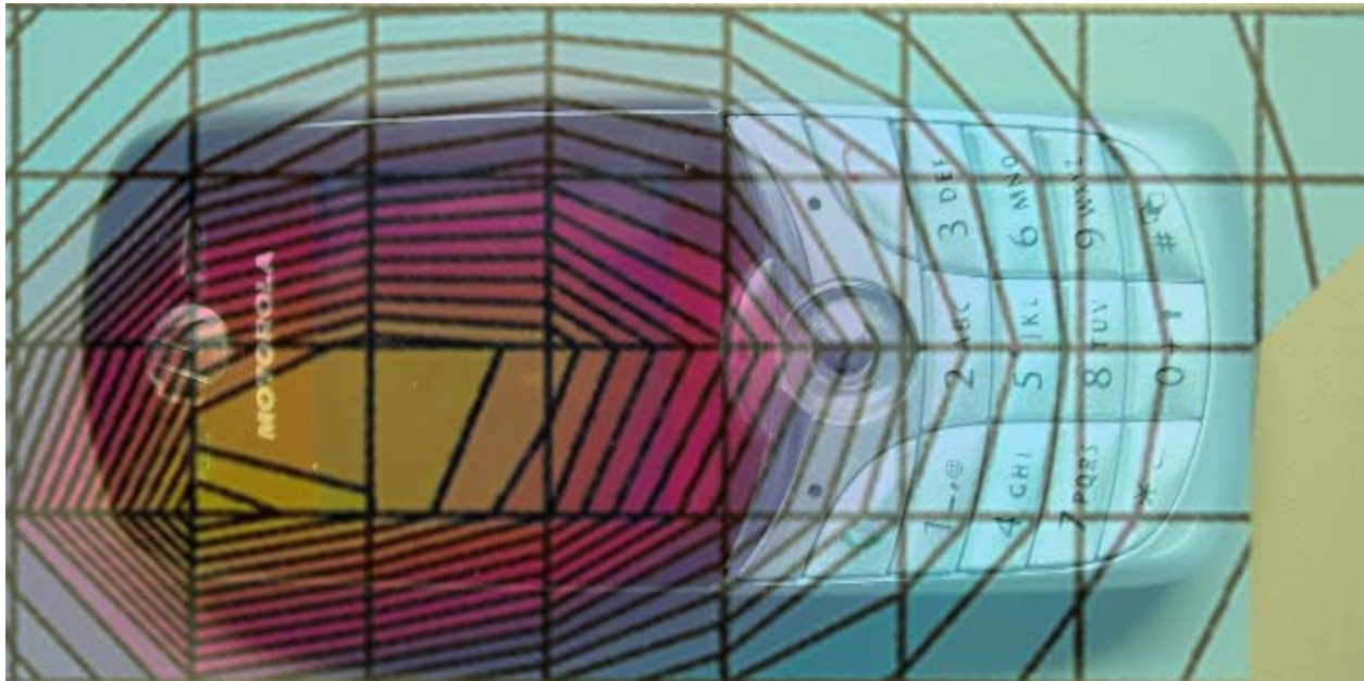
Figure 7. Typical 850MHz Right Head Adjacent Contour Overlaid on Phone with Antenna Fixed (15 ° Tilt)
