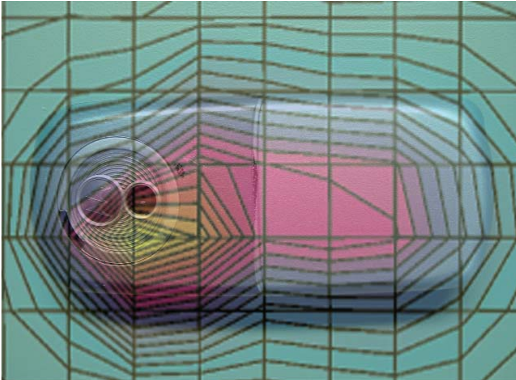
Figure 12. Typical 1900 MHz Body-Worn Contour Overlaid on Phone in Data Mode
