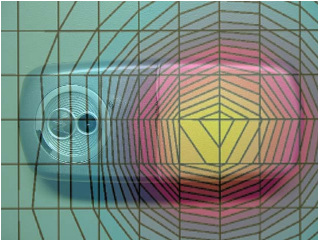
Figure 11. Typical 850 MHz Body-Worn Contour Overlaid on Phone in Data Mode
