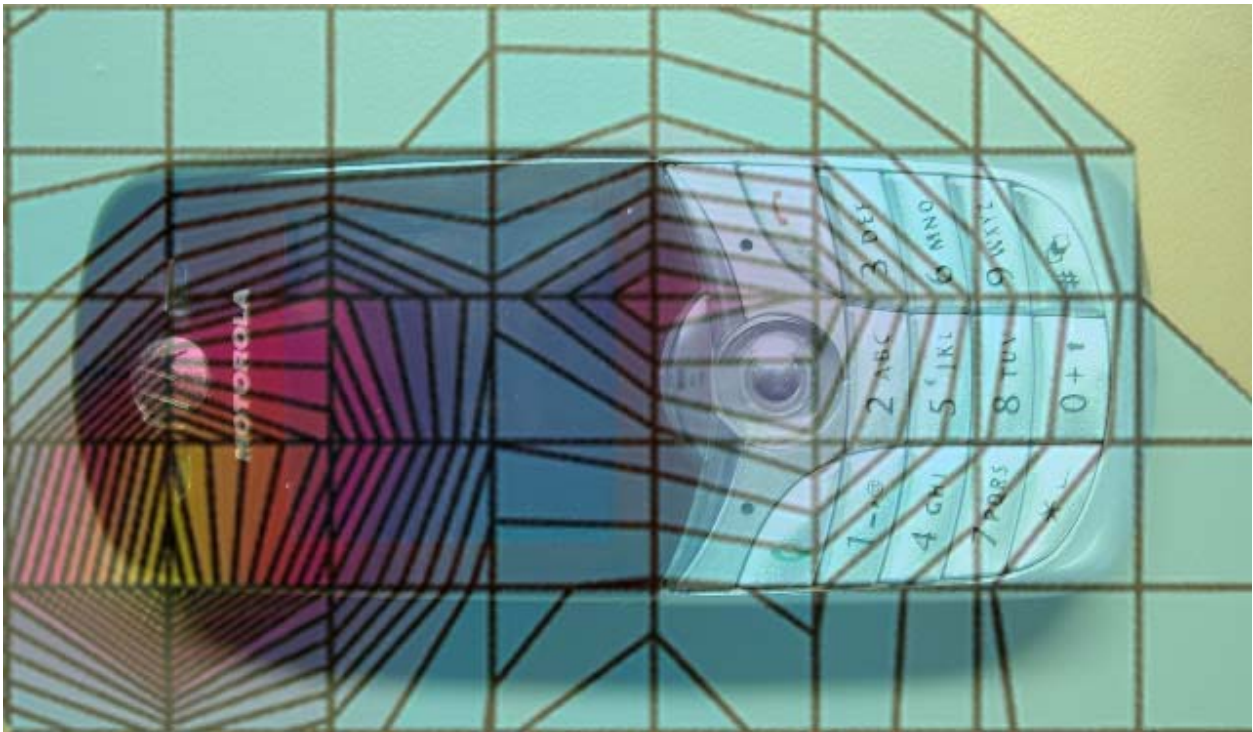
Figure 2. Typical 1900MHz Left Head Adjacent Contour Overlaid on Phone with Antenna Fixed (Cheek Touch)
