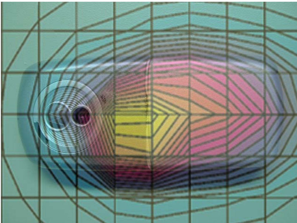
Figure 10. Typical 1900 MHz Body-Worn Contour Overlaid on Phone in Voice Mode
