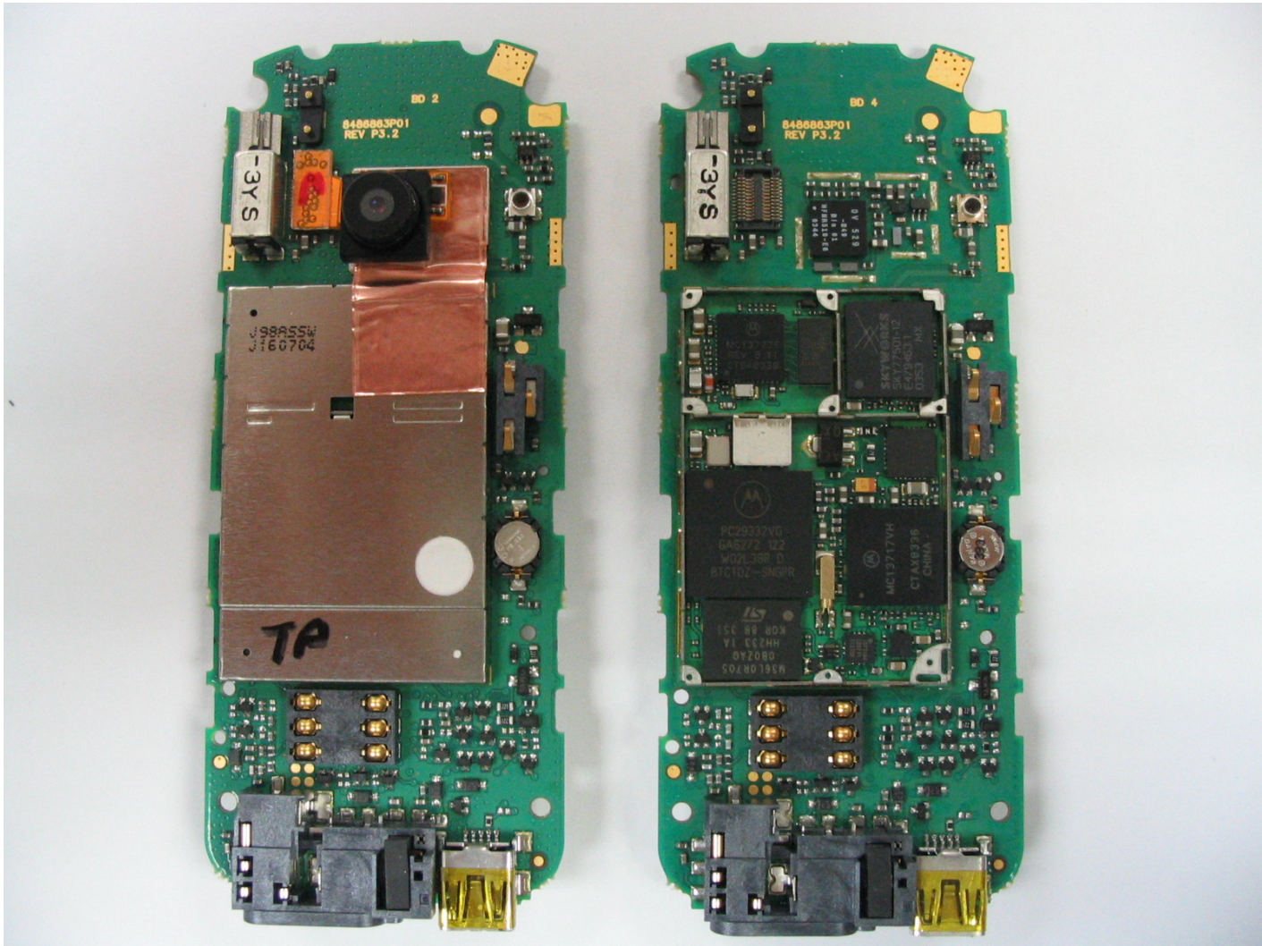
Rear View
