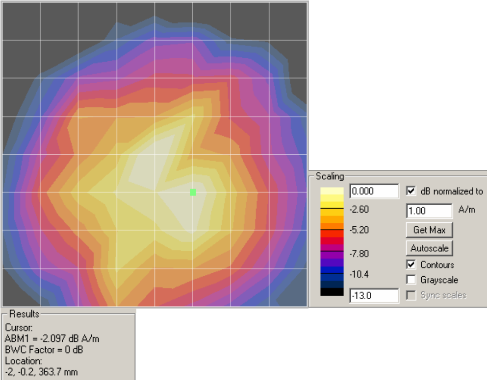
Axial – ABM1
