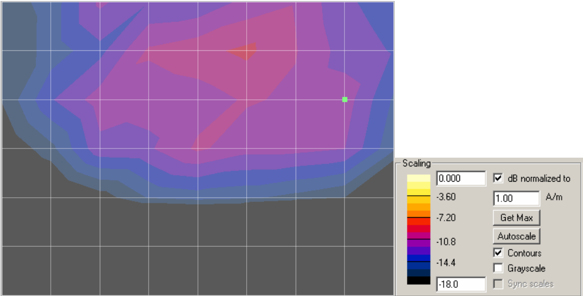
Radial 2 - ABM1
