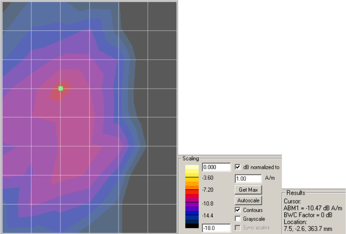
Radial 1 – ABM1
