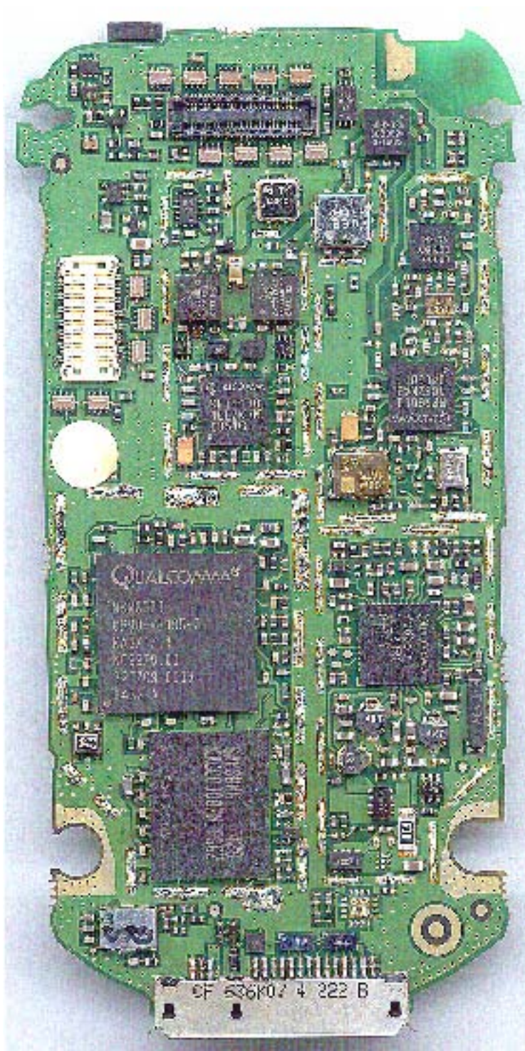
Main Board Without Shields
