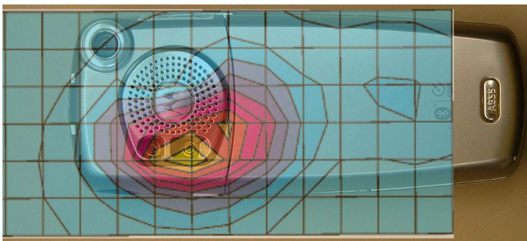
Figure 9. Typical 1900MHz W-CDMA Body Worn Contour Overlaid on Phone
