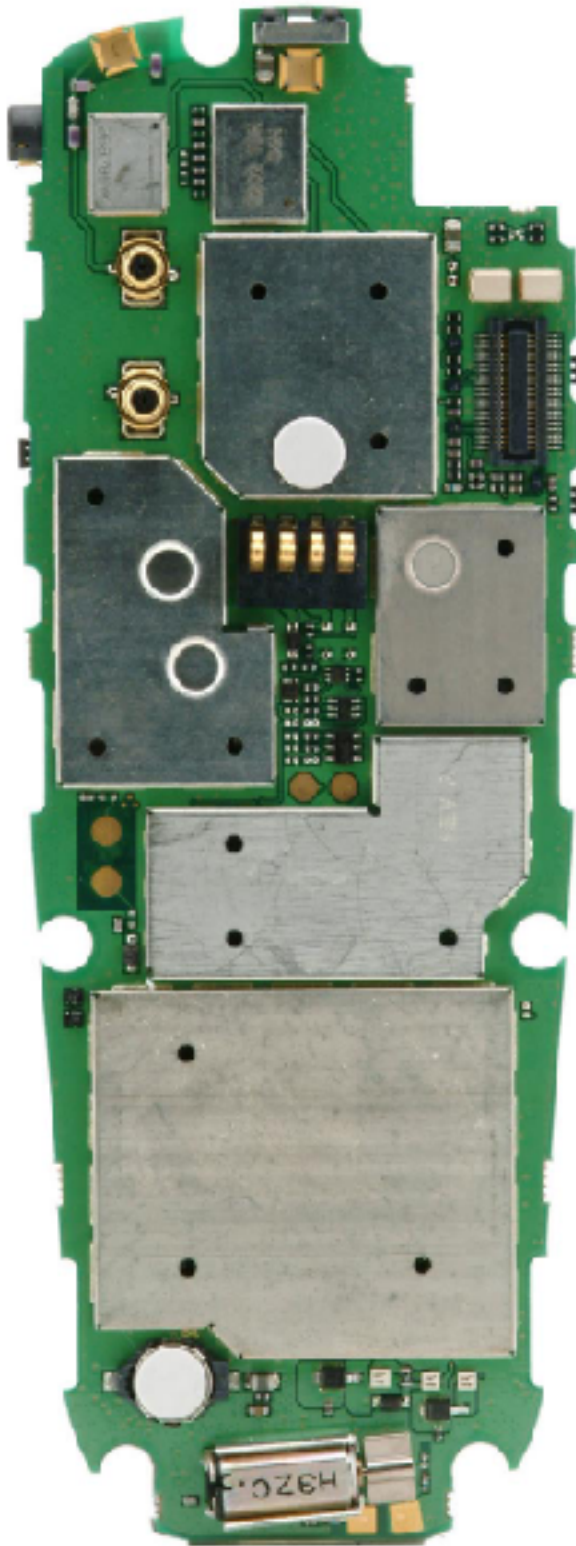
Rear View with Shields
