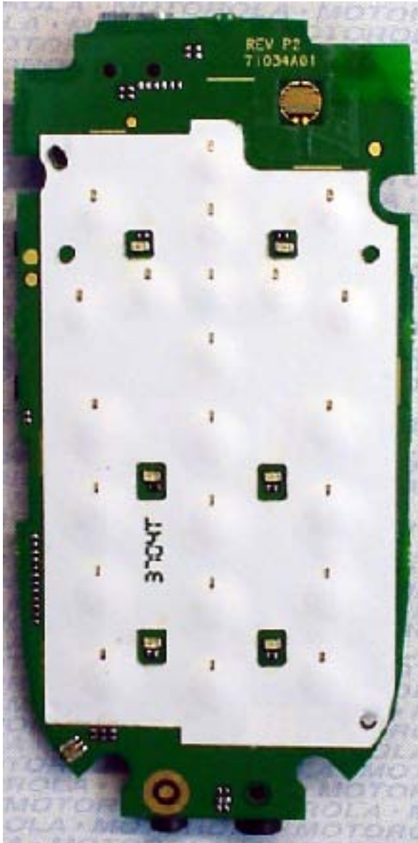
Front View with Keypad Popple
