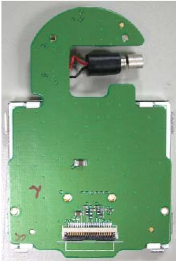
Sub Board Rear View
