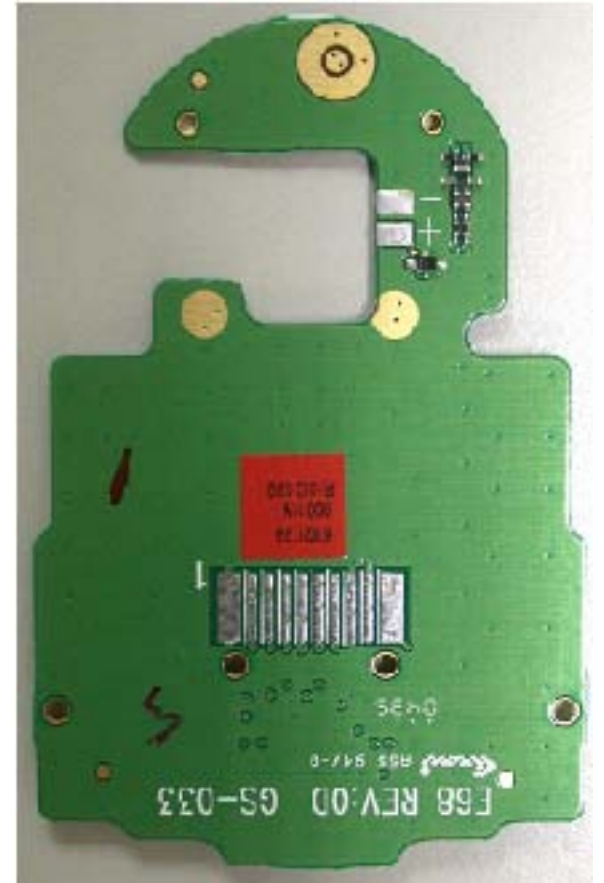
Sub Board Display Removed
