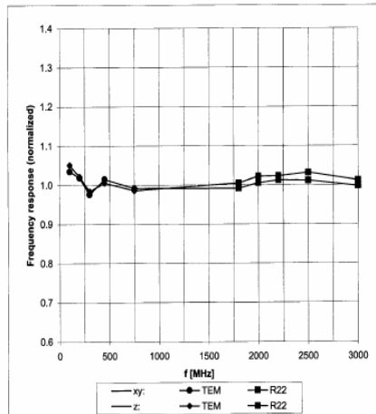
Figure 9 H-Field Probe Frequency Response
