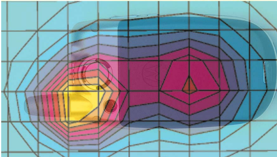
Figure 6. Typical 1900 MHz Body-Worn Contour Overlaid on Phone
