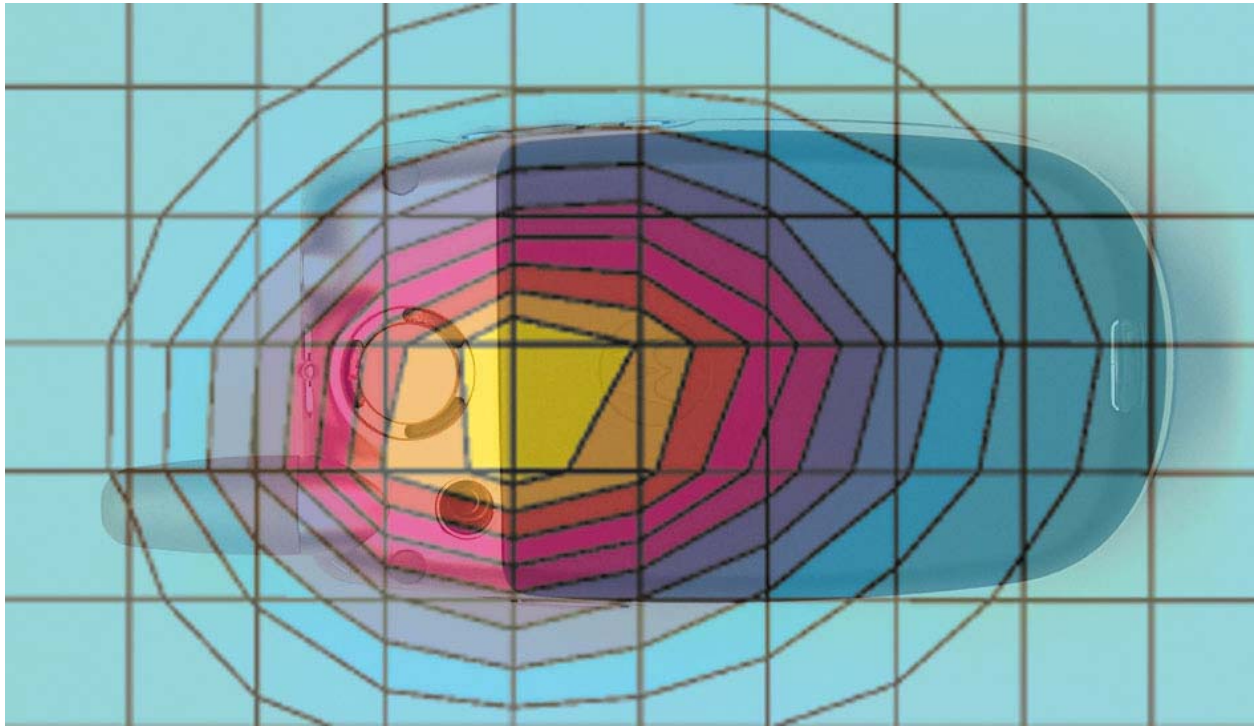
Figure 5. Typical 800 MHz Body-Worn Contour Overlaid on Phone
