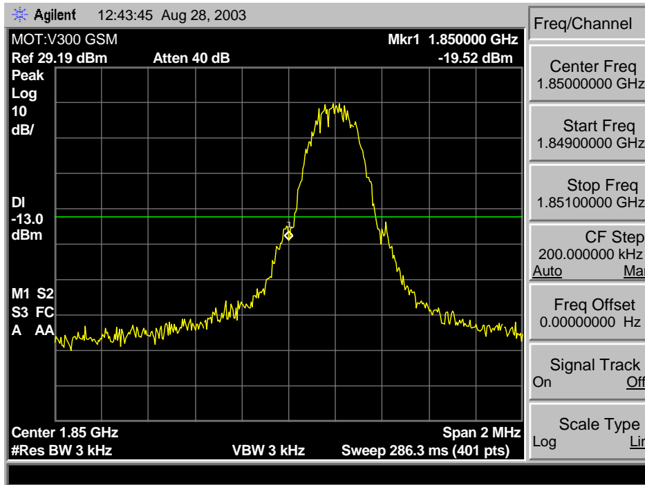
GSM 1900 Lower Band Edge
