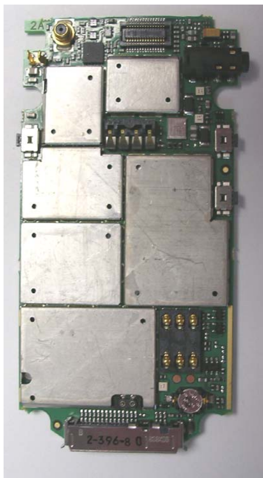
TRANSCIVER BOARD WITH RF SHIELDS
