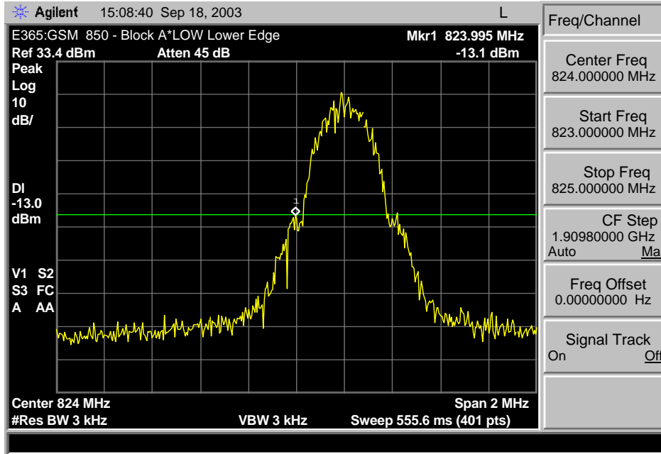
GSM 850 Lower Band Edge
