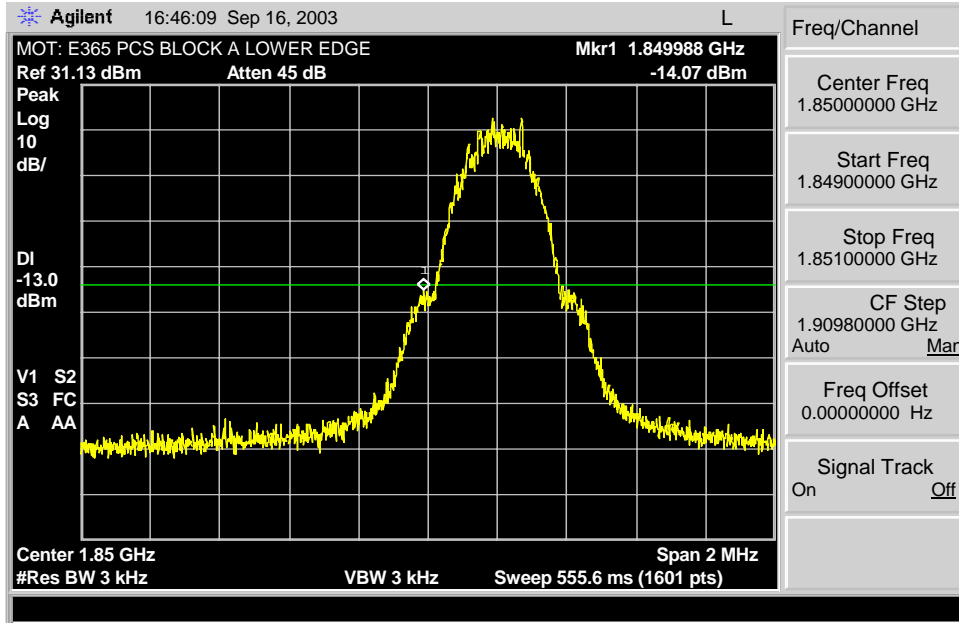
GSM 1900 Lower Band Edge
