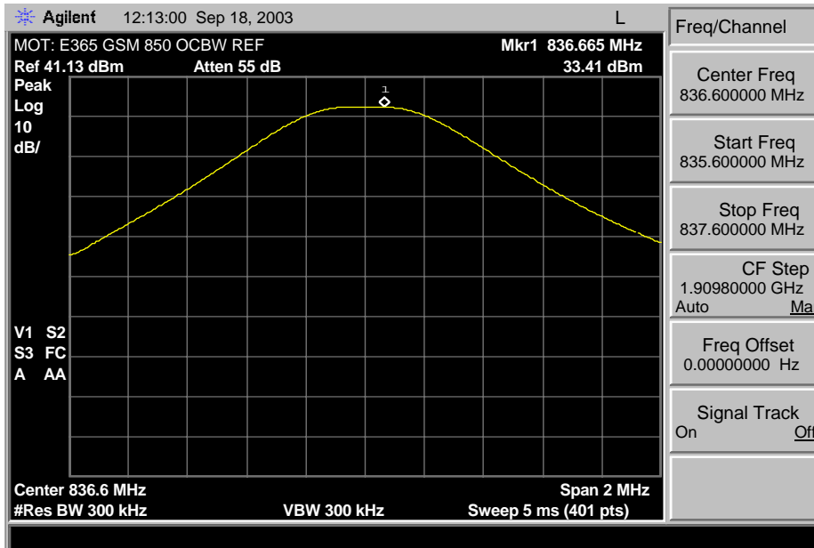
850 GSM Reference Plot
