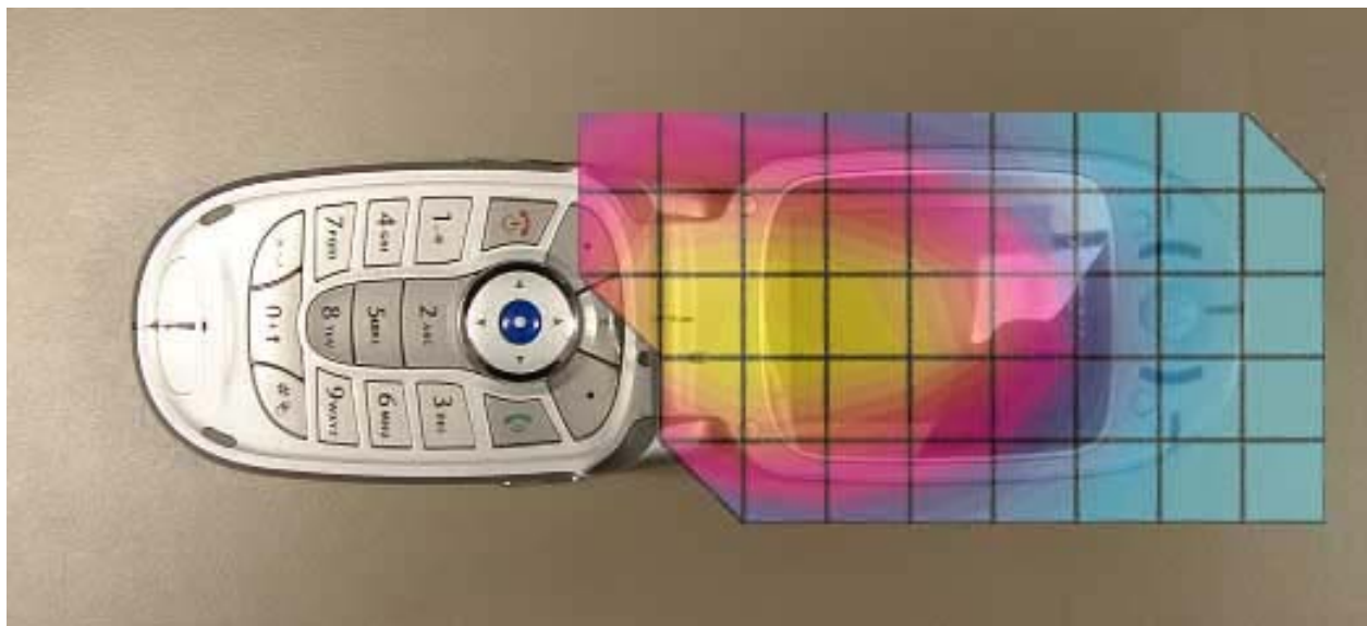
Figure 2. Typical 850MHz Left Head Adjacent Contour Overlaid on Phone with Antenna Fixed (15° Tilt)
