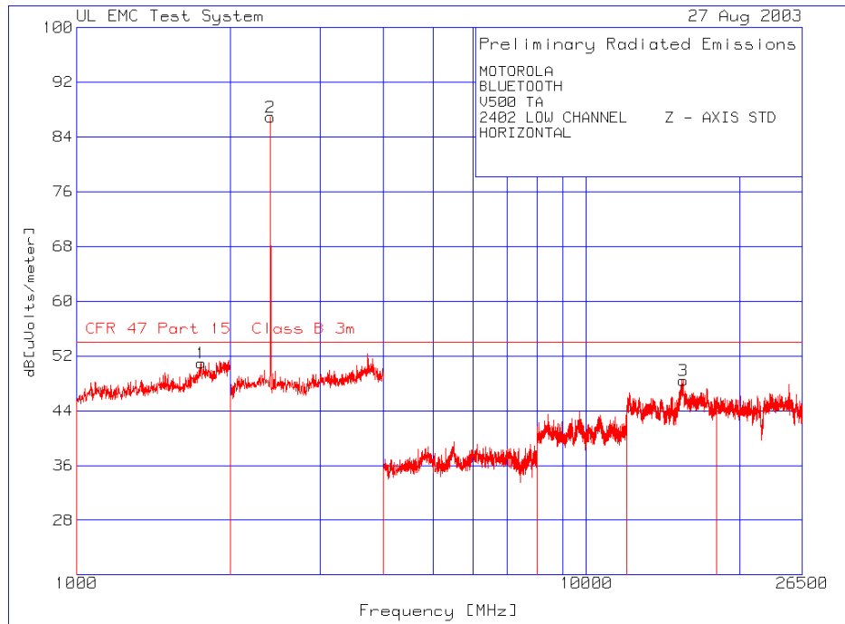
1-26.5 GHz Low Channel Horizontal
