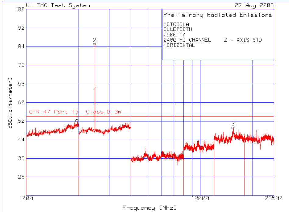
1 – 26.5 GHz High Channel Horizontal
