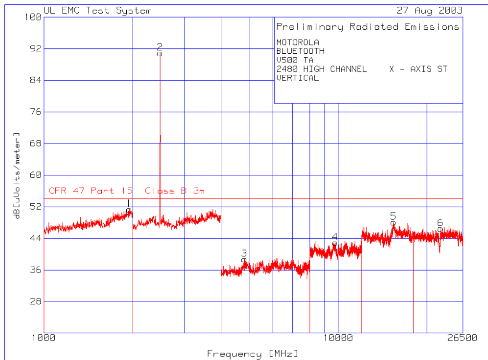
1-26.5 GHz High Channel Vertical
