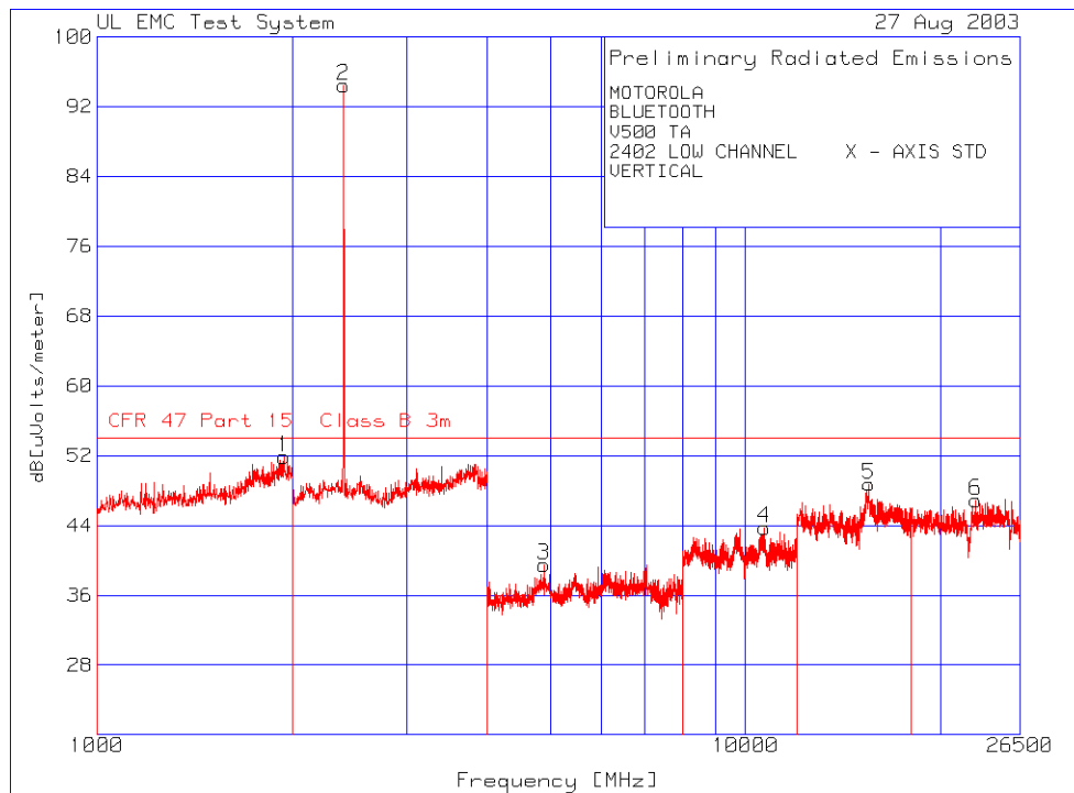
1-26.5 GHz Low Channel Vertical
