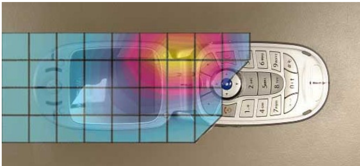
Figure 1. Typical 850MHz Right Head Adjacent Contour Overlaid on Phone with Antenna Fixed (Cheek Touch)
