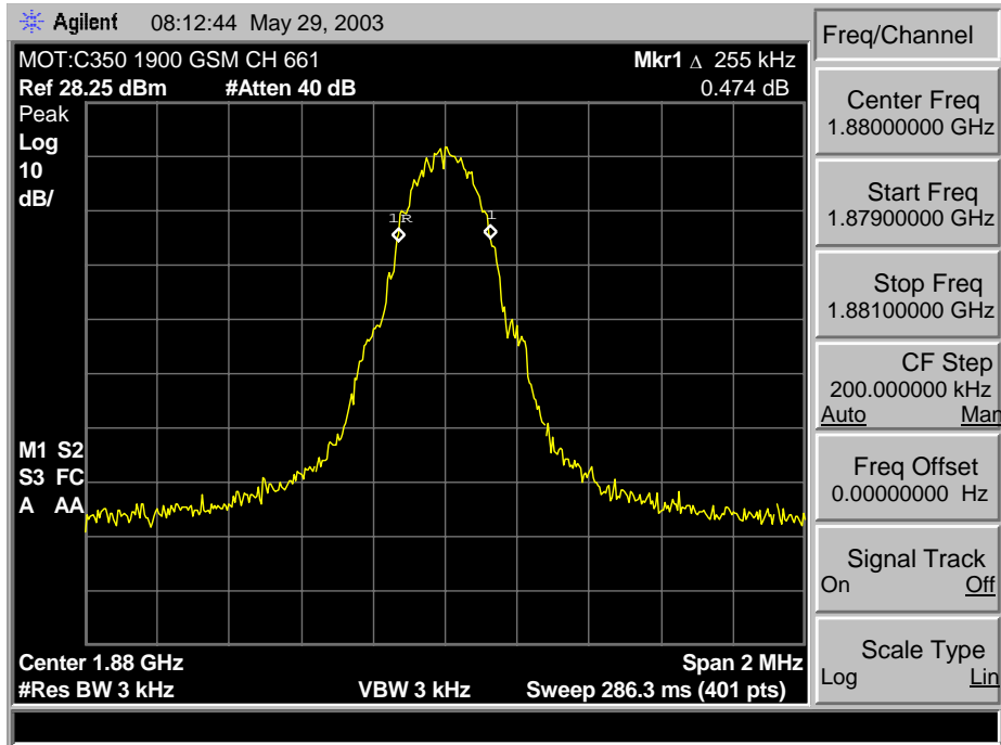
1900 GSM Occupied Band
