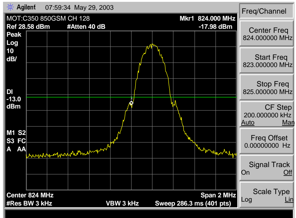
850 GSM Lower Band Edge
