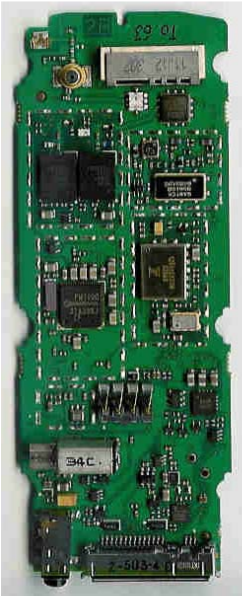
REAR VIEW (WITH SHIELDS REMOVED) MAINBOARD
