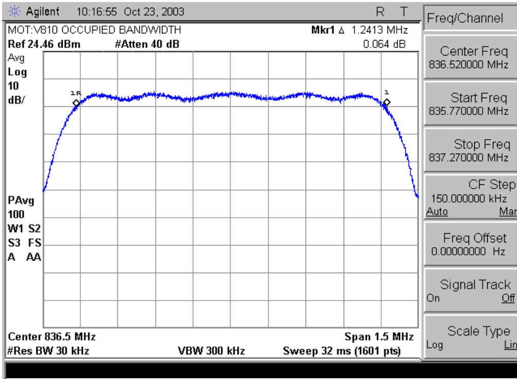
800 AMPS Occupied Bandwidth Measurement
