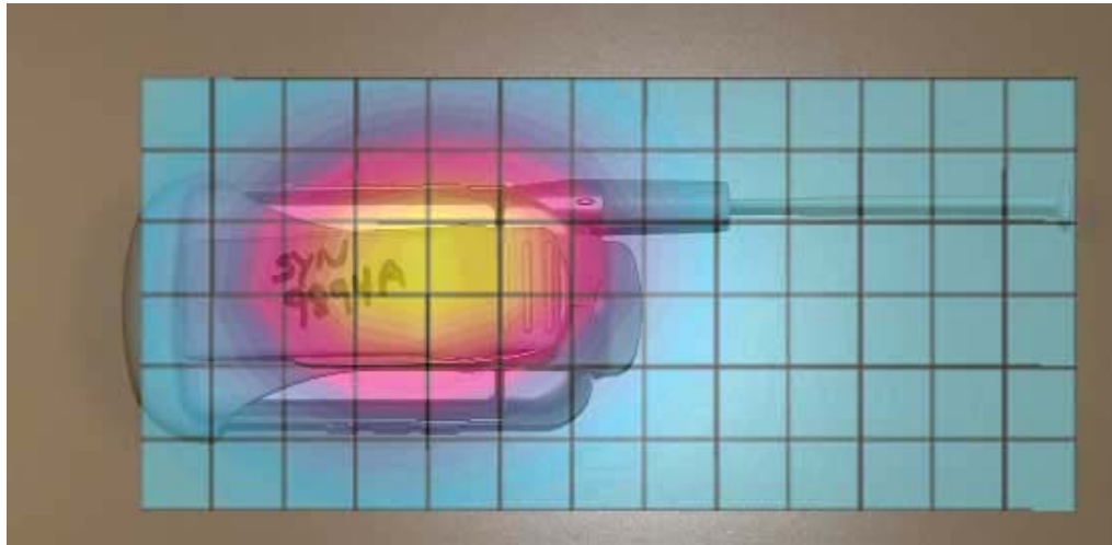
Figure 7. Typical 800 MHz Body-Worn Contour Overlaid on Phone with Antenna Extended
