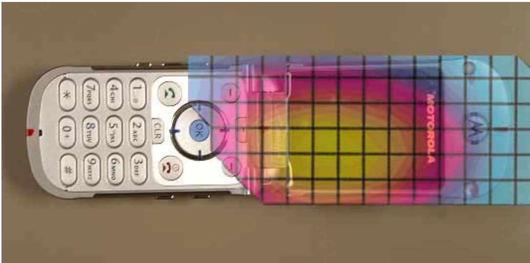
Figure 6. Typical 800MHz Left Head Adjacent Contour Overlaid on Phone with Antenna Extended (15 ° Tilt)
