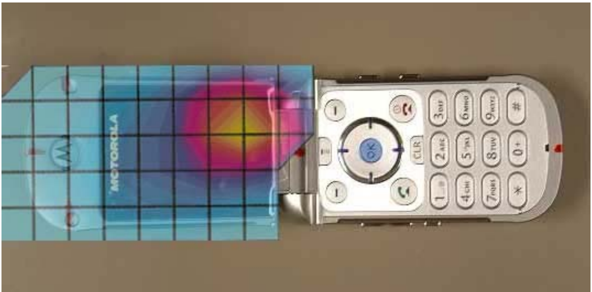
Figure 2. Typical 800MHz Right Head Adjacent Contour Overlaid on Phone with Antenna Extended (Cheek Touch)
