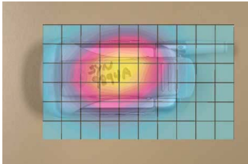
Figure 8. Typical 800 MHz Body-Worn Contour Overlaid on Phone with Antenna Retracted
