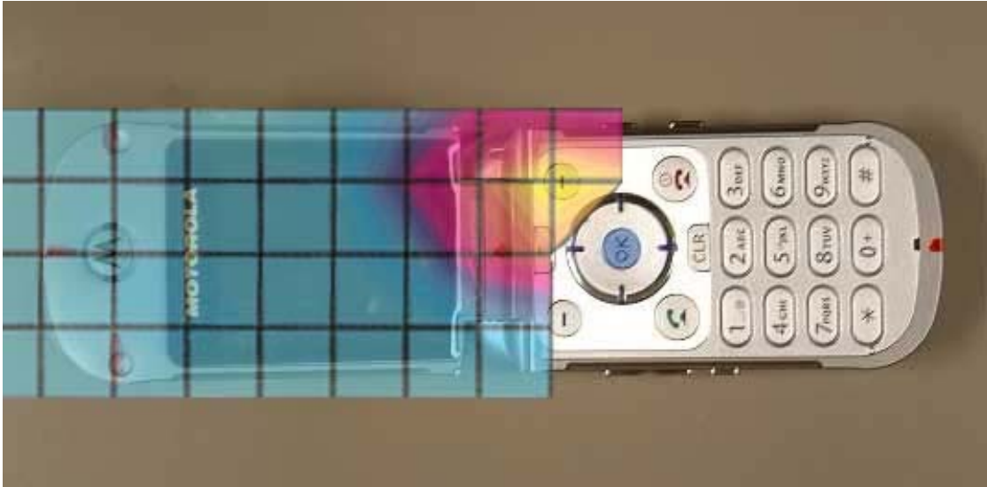
Figure 3. Typical 1900MHz Right Head Adjacent Contour Overlaid on Phone with Antenna Retracted (Cheek Touch)
