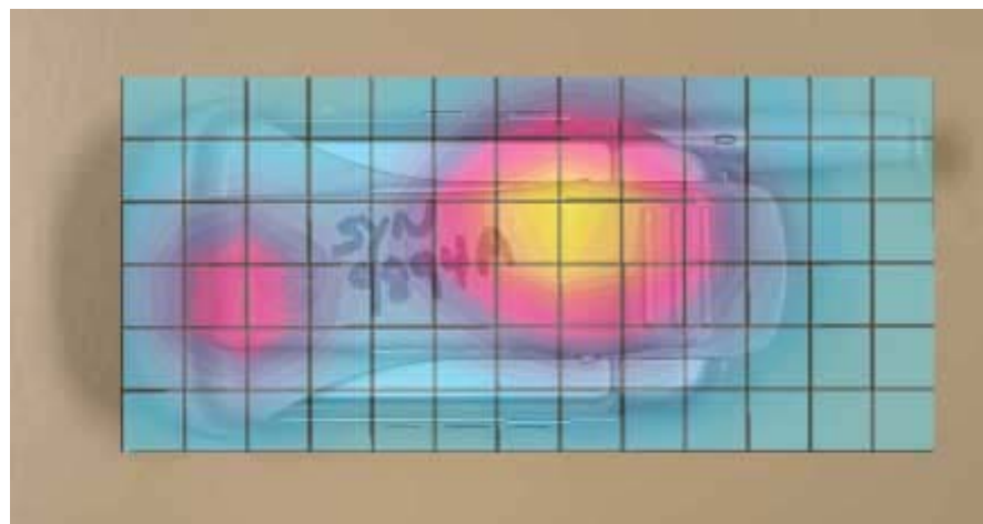
Figure 10. Typical 1900 MHz Body-Worn Contour Overlaid on Phone with Antenna Extended
