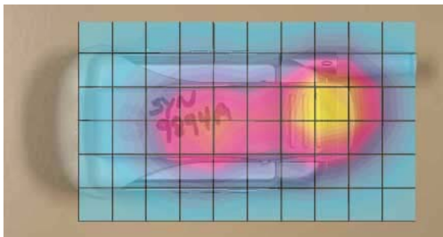
Figure 9. Typical 1900 MHz Body-Worn Contour Overlaid on Phone with Antenna Retracted
