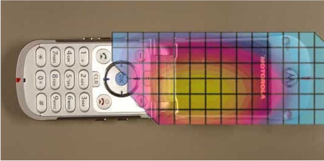
Figure 5. Typical 800MHz Left Head Adjacent Contour Overlaid on Phone with Antenna Retracted (15 ° Tilt)
