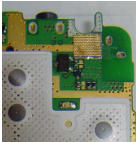
Original PCB showing hand-placed pad
