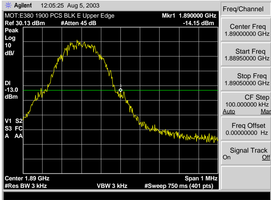
GSM 1900 E Max. Block Edge
