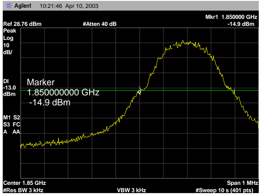
1900 GSM Lower Band Edge
