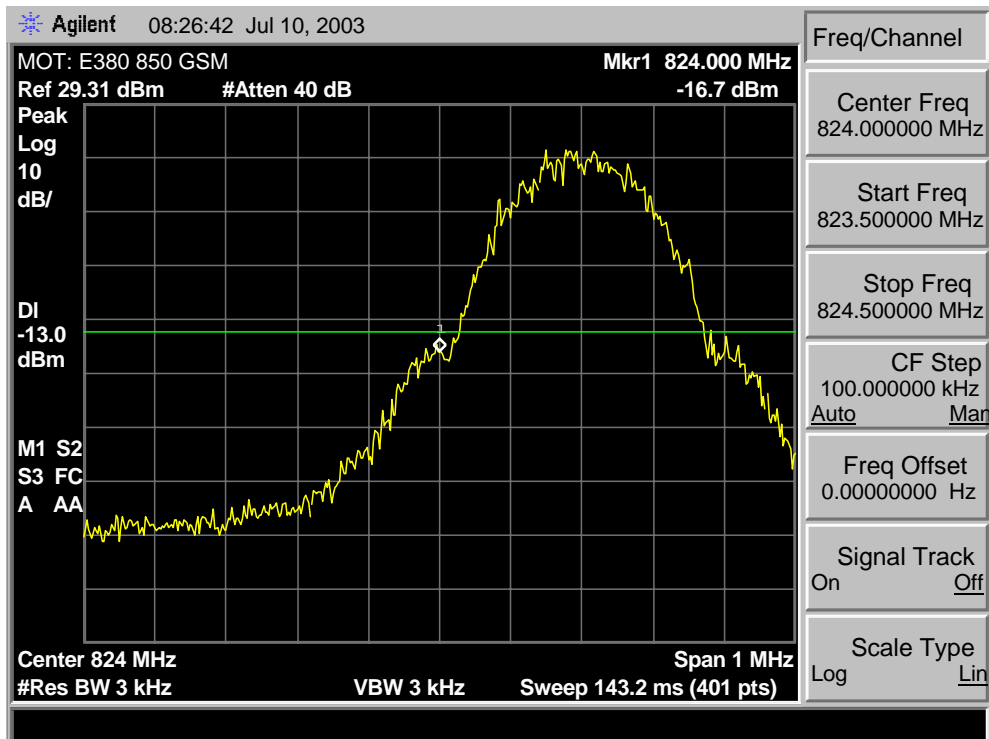
850 GSM Lower Band Edge
