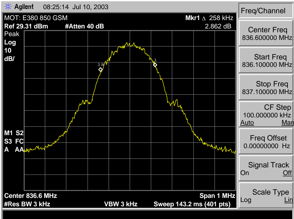
850 GSM Occupied Band
