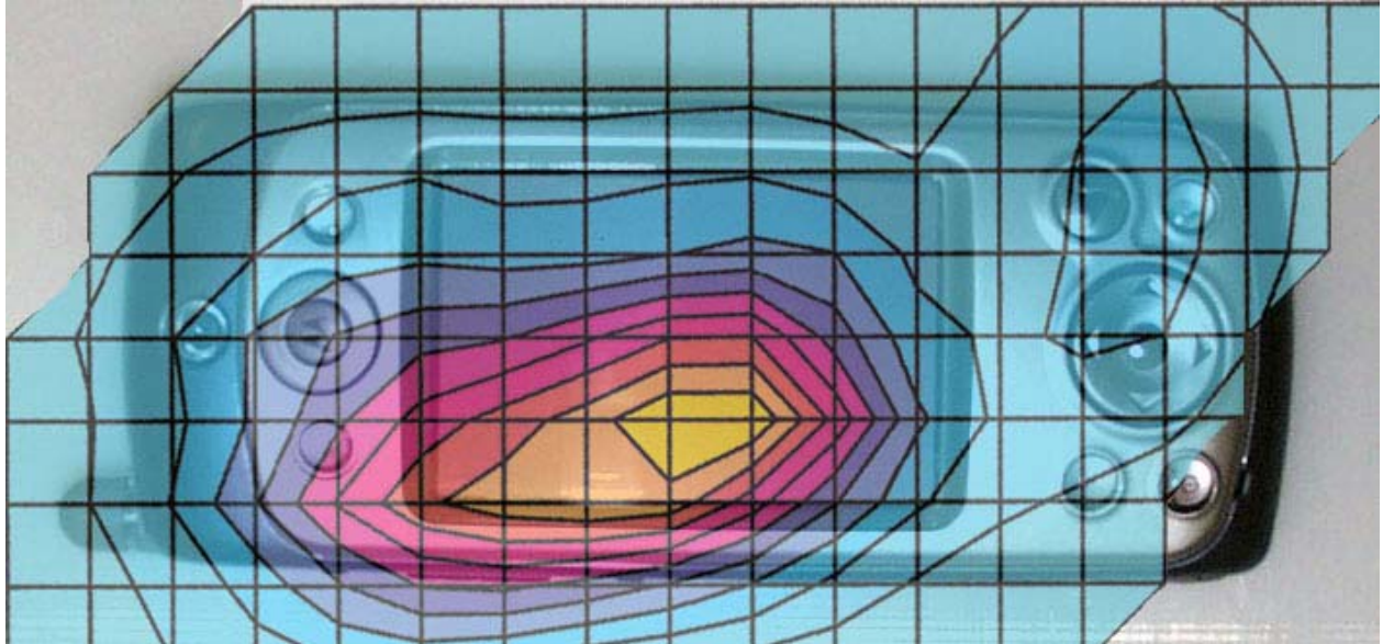
Figure 1. Typical 1900MHz Head Adjacent Contour Overlaid on Phone (Cheek Touch)
