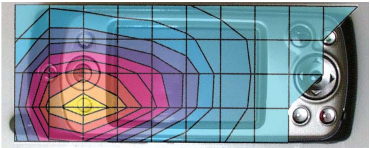
Figure 2. Typical 1900MHz Head Adjacent Contour Overlaid on Phone (15 ° Tilt)
