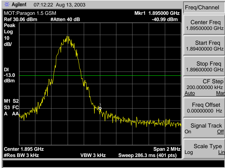
GSM 1900 C, C2, C3 Max Block Edge
