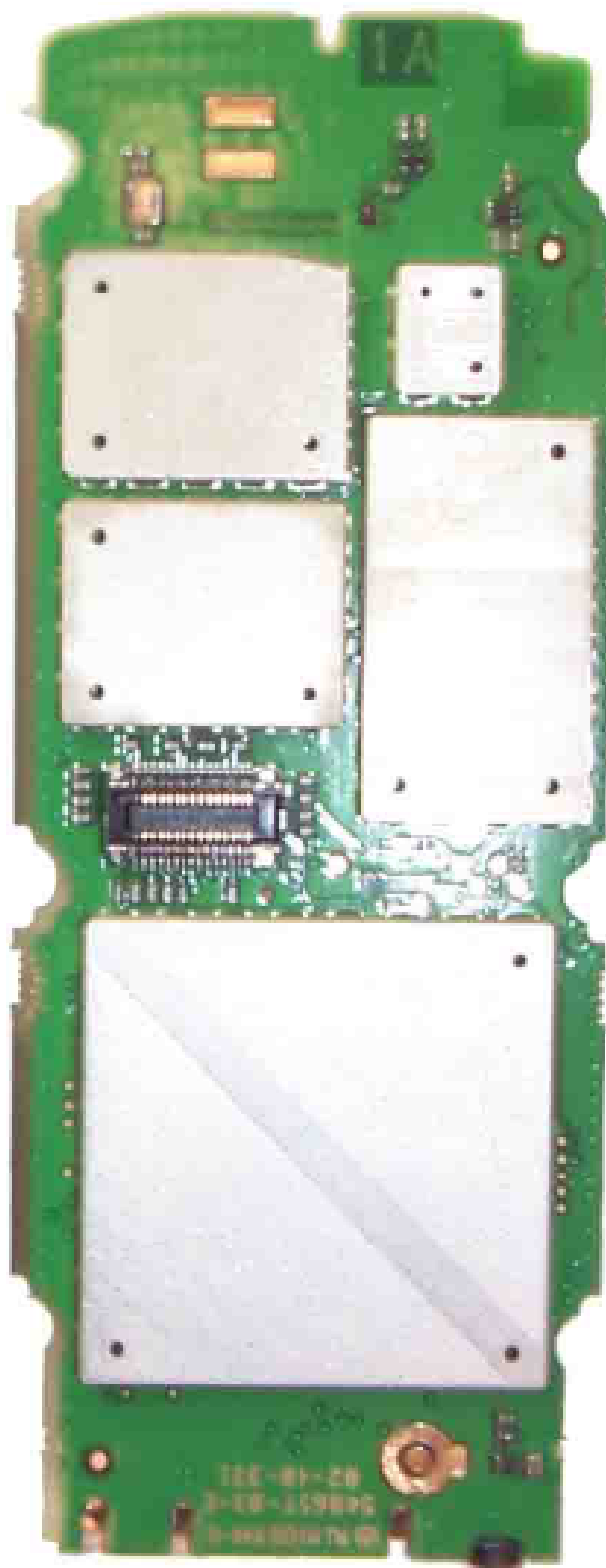
Front View
