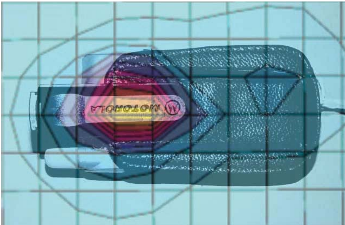
Figure 6. Typical 1900 MHz Body-Worn Contour Overlaid on Phone with Body Worn Accessory # INT720D1
