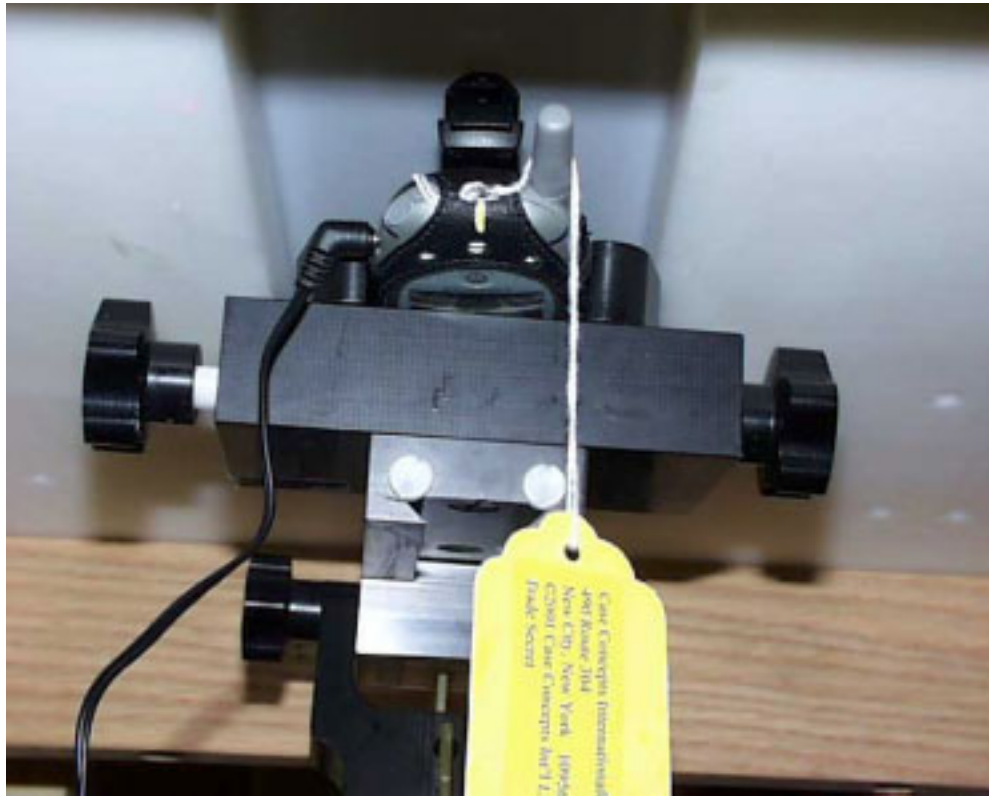
Figure 15. Phone with leather pouch with universal belt clip Placed under a Flat Phantom with Headset (Antenna Fixed)
