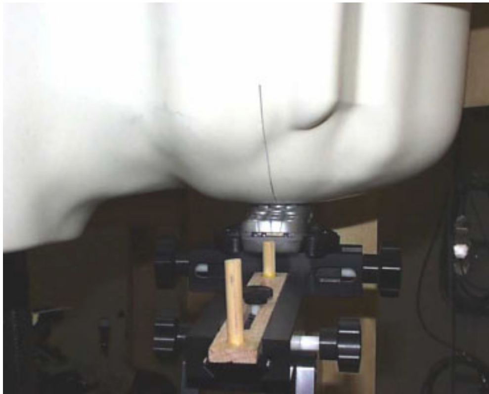
Figure 11. Front View of Phone Placed Against Head with Antenna Fixed
