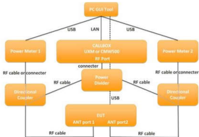
Figure 6- 2 TA-SAR conductive power test setup block diagram for scenarios 6/7
