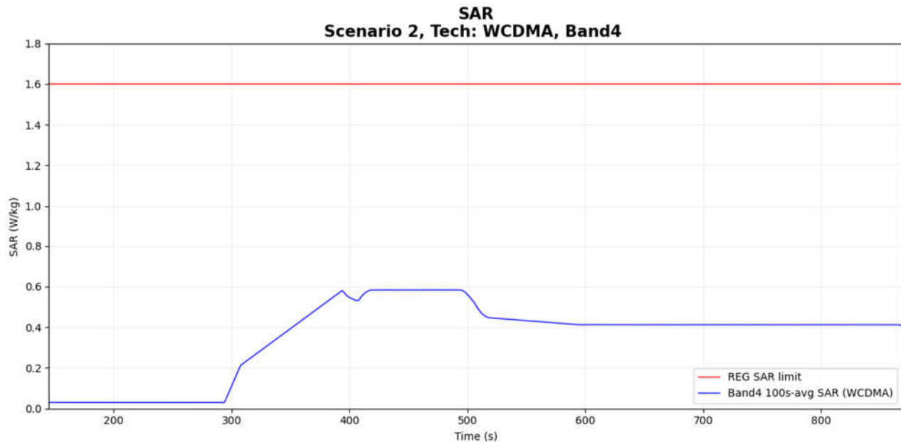
Figure 7-2 Time-averaged SAR
