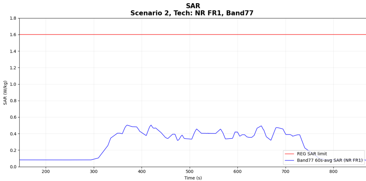
Figure 7-13 Time-averaged SAR for case
