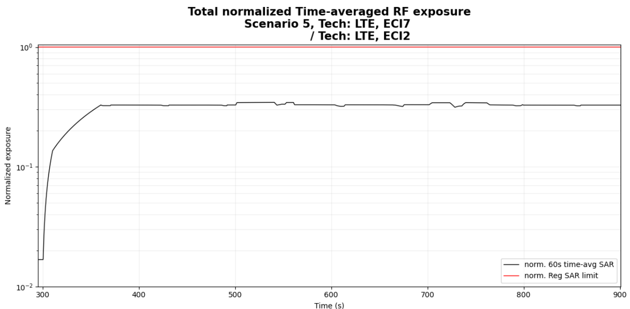
Figure 6- 19 Normalized time-averaged SAR
