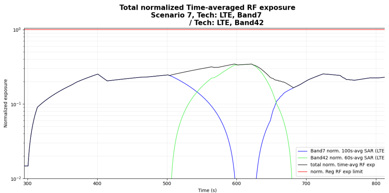
Figure 6- 21 Normalized time-averaged SAR
