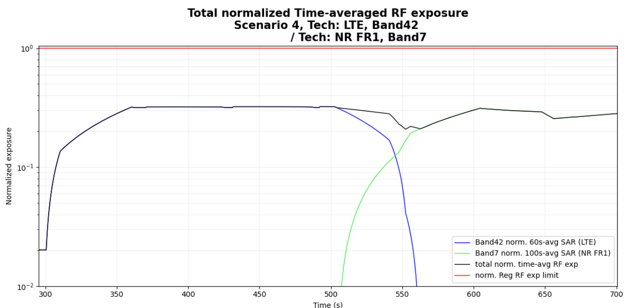
Figure 6- 18 Normalized time-averaged SAR
