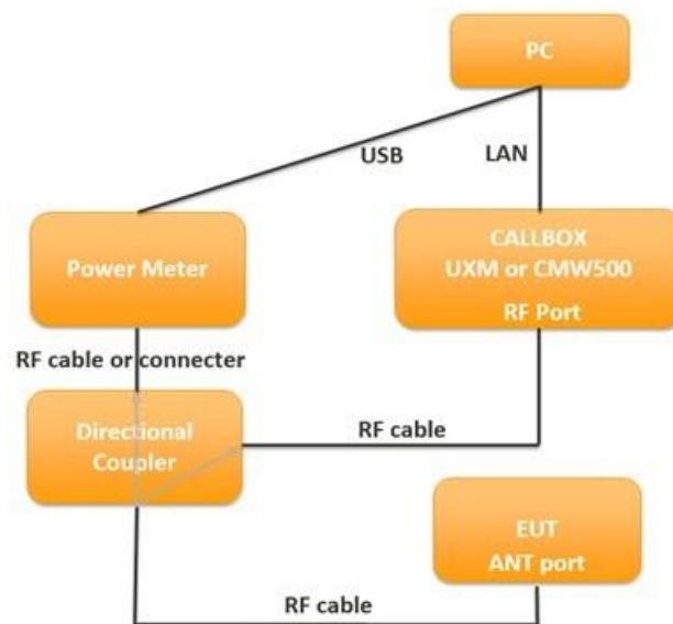
Figure 6- 1 TA-SAR Gen2 conductive power test setup block diagram for scenarios 1/2/3/5
