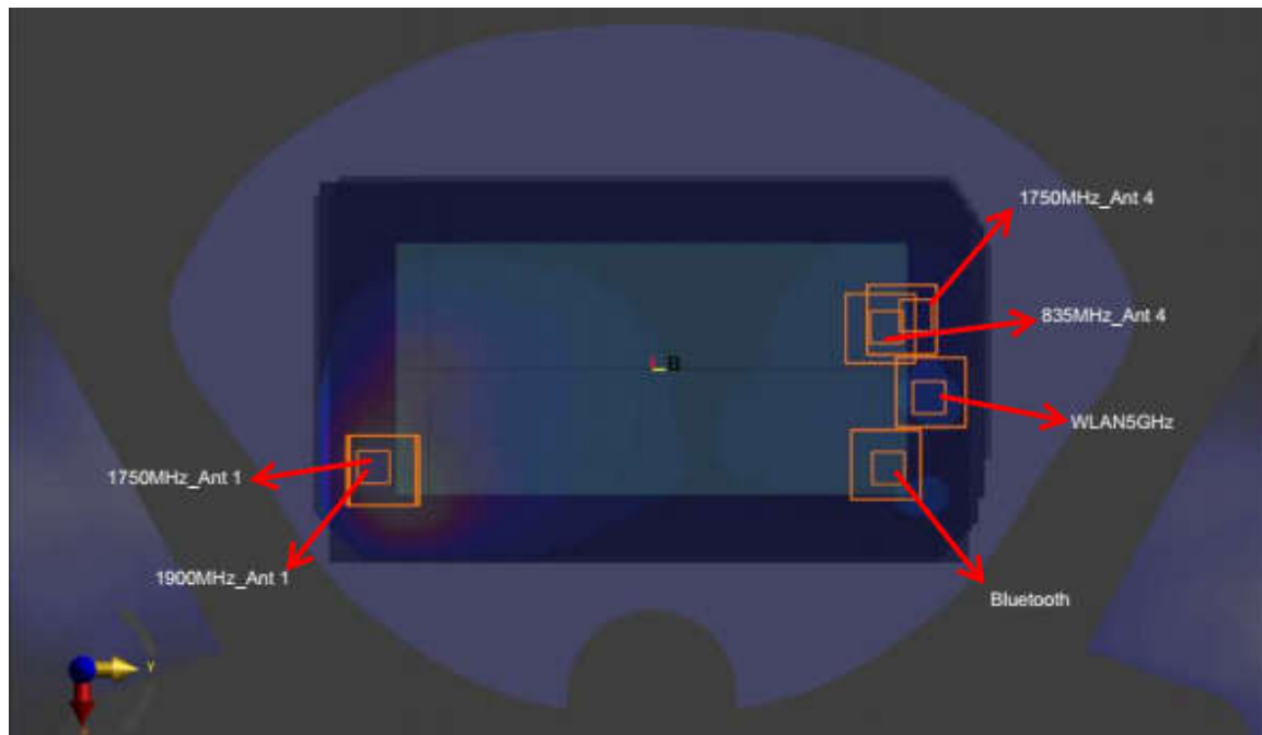
ULCA+WLAN5GHz+BT_Body Worn_Front_5mm
