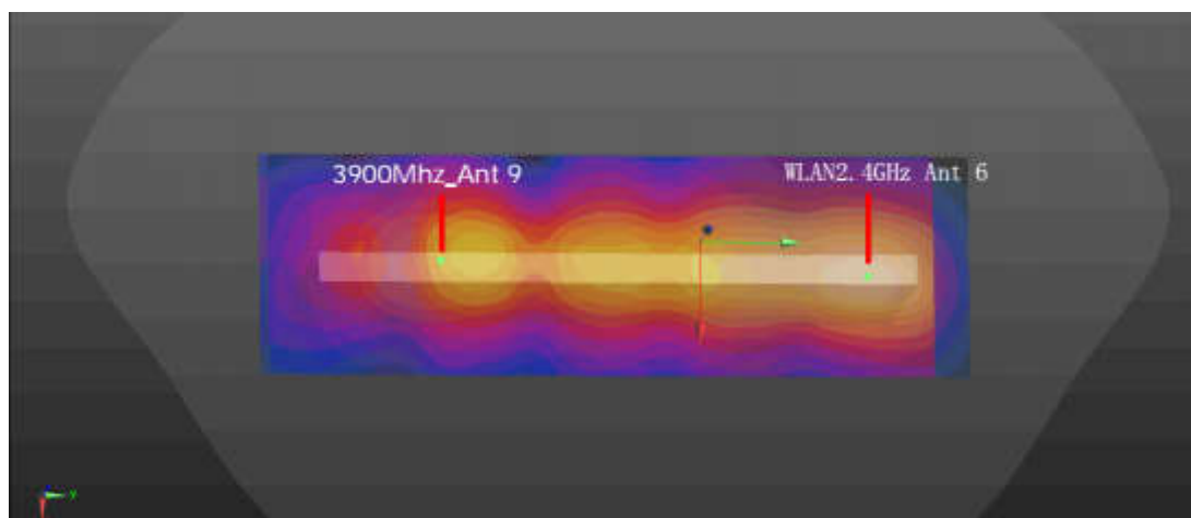
WWAN+WLAN_Hotspot_Right Side_5mm
