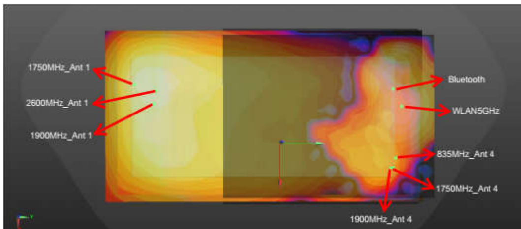
ULCA+WLAN5GHz+BT_Body Worn&Hotspot_Back_5mm
