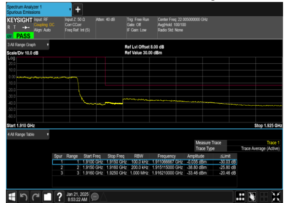
N25(20M)_DFT-s-OFDM_QPSK_Outer_Full_High_CH
