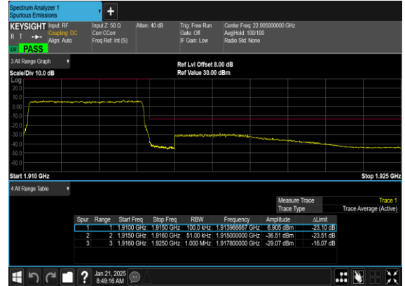
N25(5M)_DFT-s-OFDM_QPSK_Outer_Full_High_CH
