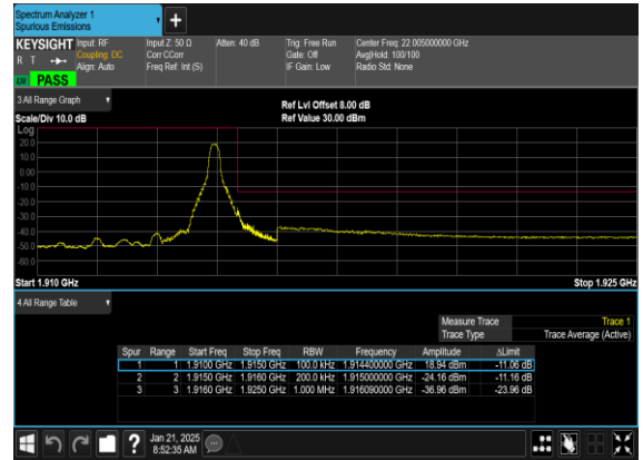
N25(20M)_DFT-s-OFDM_QPSK_Edge_1RB_Right_High_CH
