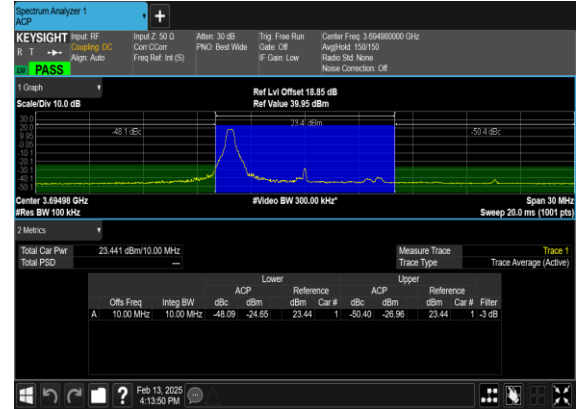
N48(10M)_DFT-s-OFDM_PI_2-BPSK_Edge_1RB_Left_High_CH
